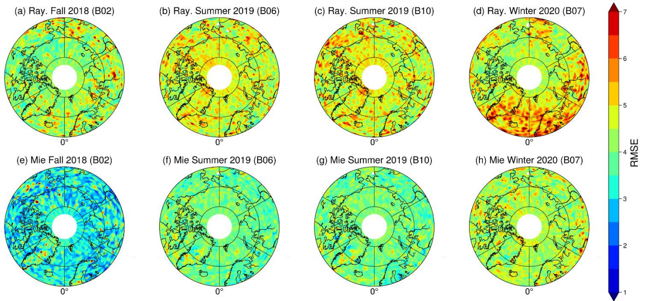
Figure 4011. RMSD of Aeolus and ECCC-B vertical HLOS wind profiles for selected lower-atmospheric regions (Rayleigh T and Mie B+T) during fall 2018, summer 2019, and winter 2020.
