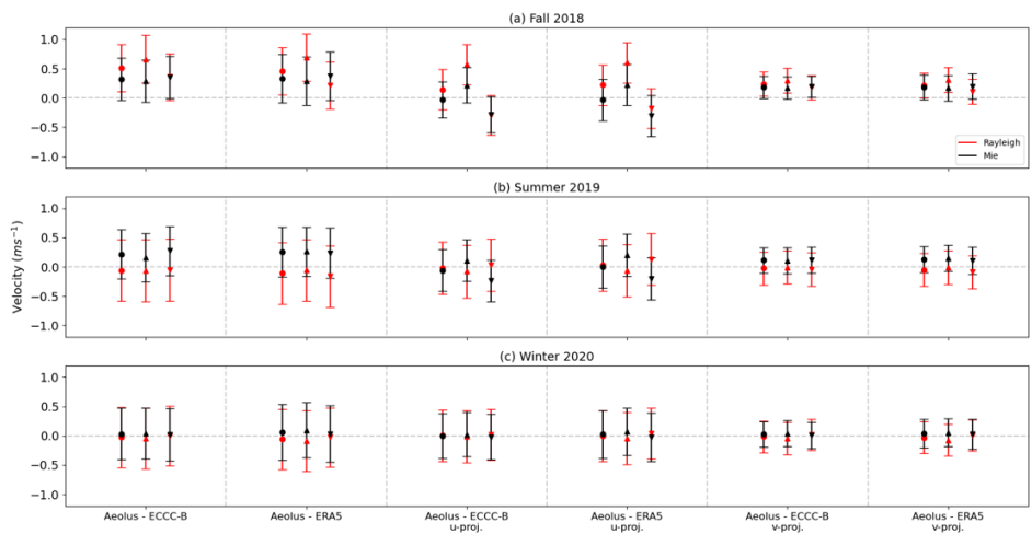
Figure 89. Means ( 10^0 ) and standard deviations ( 10^1 ) of the distributions of the differences between Aeolus Rayleigh (Mie) winds and ECCC-B and ERA5 shown as red (black) dots or triangles, and error bars, over the Arctic during (a) boreal fall 2018, (b) summer 2019, and
