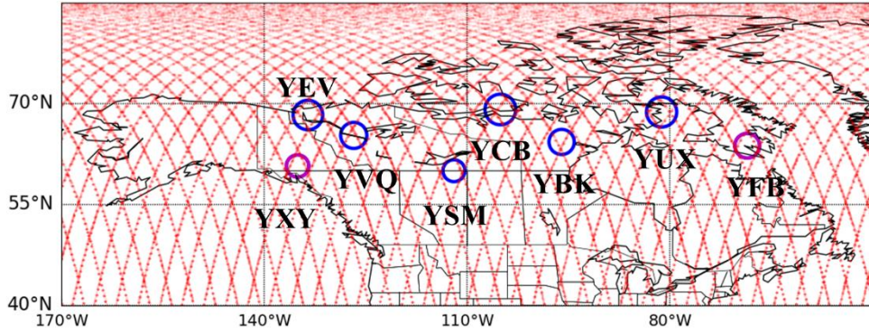
Figure 1. Aeolus's overpasses centred over northern Canada the Canadian North (red dots) during the first week of August 2019. The magenta green 90-km radius circles centred on Iqaluit (YFB) and Whitehorse (YXY) within which coincident Aeolus overpasses were compared with other datasets (some circles appear differently sized because of map projection distortion) . The blue circles indicate the locations of other radiosonde stations over the Canadian Arctic: Inuvik (YEV), Fort Smith (YSM), Hall Beach (YUX), Cambridge Bay (YCB), Norman Wells Ua (YVQ), and Baker Lake (YBK).
