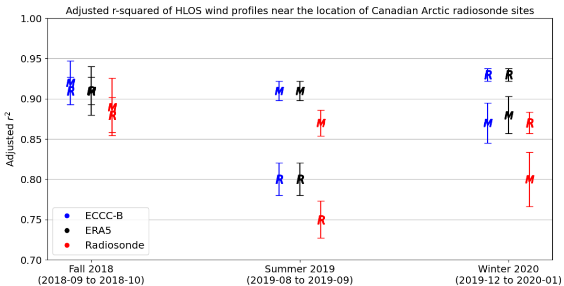
Figure 56. Adjusted r-squared of vertical HLOS wind profiles with 99% confidence level from coincident Aeolus (Rayleigh, R, and Mie, M) overpasses near radiosonde stations over the Canadian Arctic (shown in Figure 1) and ECCC-B, ERA5, and radiosonde measurements during fall 2018 (early FM-A), summer 2019 (early FM-B), and winter 2020 (mid-FM-B).
