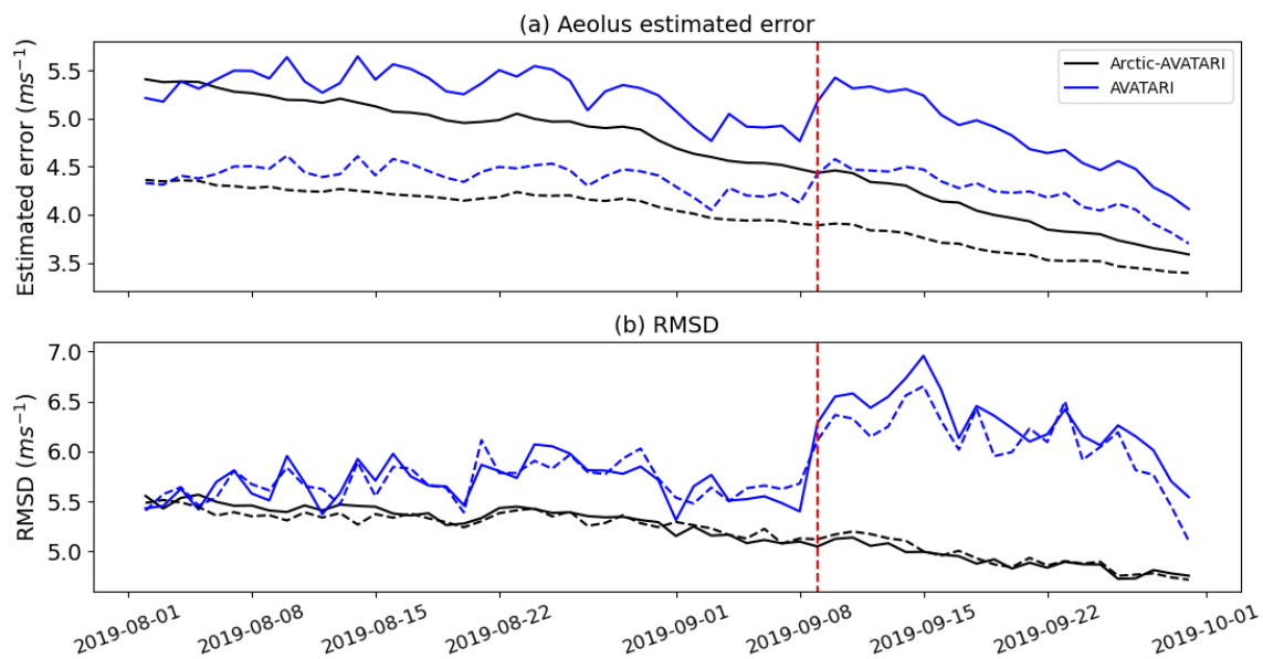
Figure 67. Time-series of (a) Aeolus L2B estimated error of Rayleigh winds and (b) RMSD between the ECCC-B and Aeolus 2B06 (solid) and 2B10 (dashed) data from 2 August to 30 September 2019. The data is averaged over the region with a different range bin setting for the AVATAR-I campaign (blue) and over the rest of the Arctic (black).
