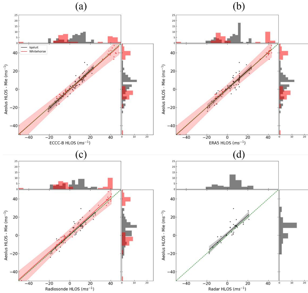
Figure 5. Similar to Figure 34, but scatter plots between Aeolus Mie winds and other datasets.
