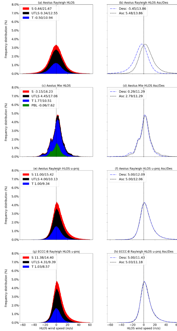
Figure 78. Aeolus Rayleigh ((a) and (b)) and Mie ((c) and (d)) HLOS measurement stacked frequency distributions (%) during winter 2020 over the Arctic ( >70^\circ N). The HLOS winds are projected onto the east-west directions ((e) to (h)) from Aeolus Rayleigh measurements and ECCC-B HLOS winds. The panels on the right show the distribution of ascending and descending measurements separately. The means and standard deviations of distributions in each atmospheric layer are listed in the figure legends.
