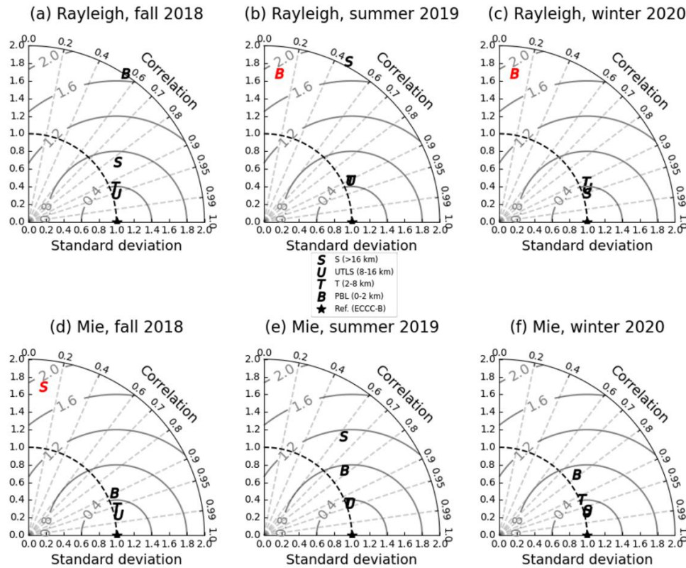
Figure 910. Normalized Taylor diagrams with ECCC-B as references for Aeolus measurements over the Arctic. The correlation coefficients and standard deviations are calculated for each layer. The angle indicates the correlation between Aeolus measurements and the reference. The distance to the origin represents the normalized standard deviation and to the star (reference) represents the normalized root-mean square error. Rows are distinguished by channels; columns are distinguished by seasons. The red markers on top left of panels represent layers with normalized standard deviations that are outside the range shown (> 2.2).
