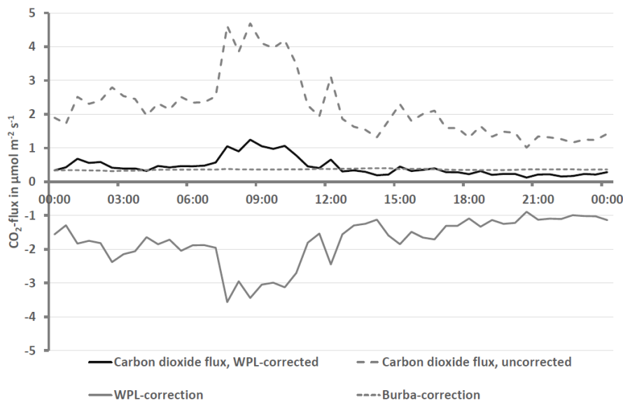
Figure 1: Comparison of WPL-corrected and uncorrected \text{CO}_2 -flux together with the size of the WPL- and Burba-correction on 06 December 2015 at the Bayelva site calculated with EddyPro, temperature range 268–270 K
