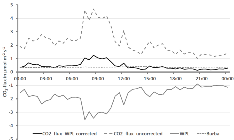
75 Figure 1: Comparison of WPL-corrected and uncorrected CO 2 -flux together with the size of the WPL- and Burba-correction on 06 December 2015 at the Bayelva site calculated with EddyPro
