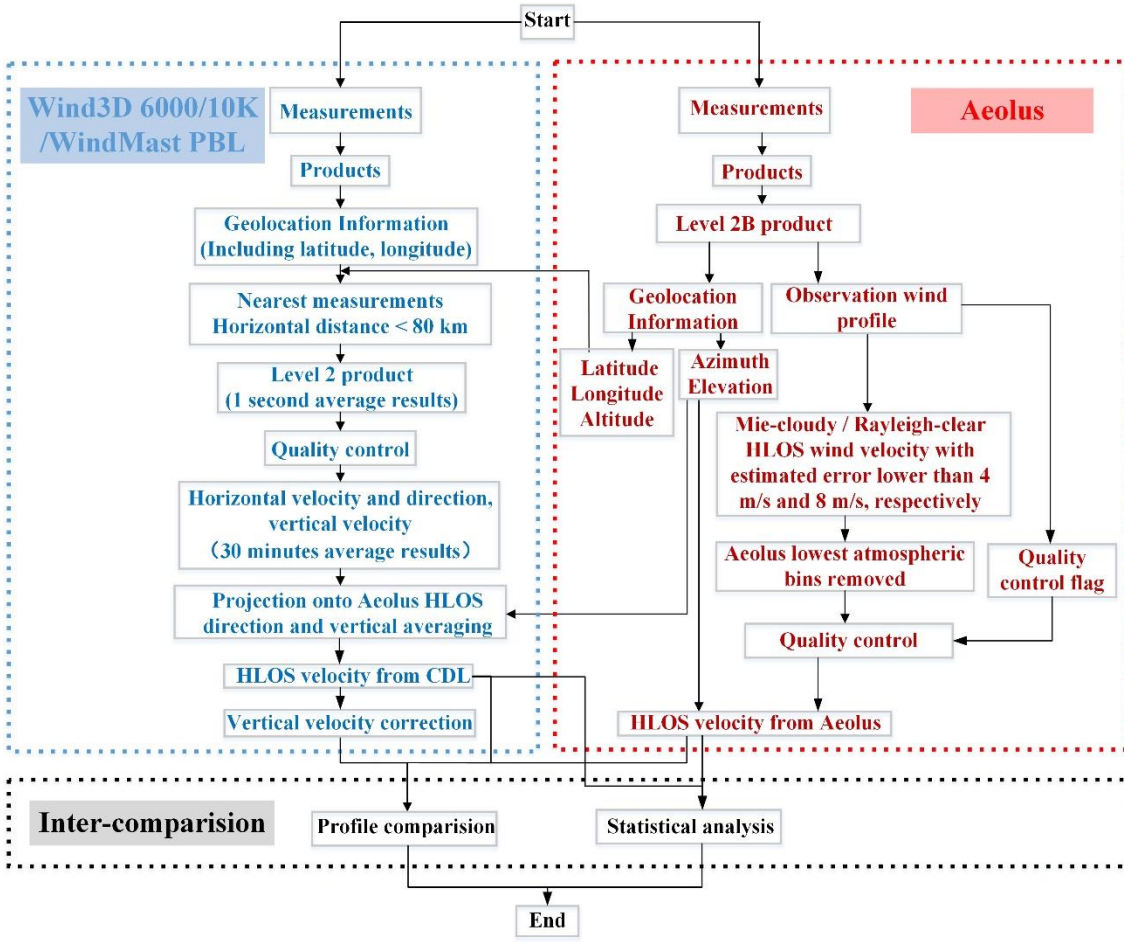
Figure 4. Sketch of the comparison between CDL and Aeolus in the atmospheric boundary layer.
