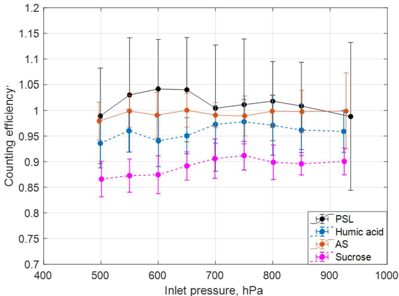
Fig. 8, CPC 3789 counting efficiency at different operating pressure with four different types of 100 nm aerosol particles (PSL, humic acid, AS, and sucrose), when the temperature conditions are T_{\text{cond}} = 27^\circ\text{C} and T_{\text{ini}} = 59^\circ\text{C} .
