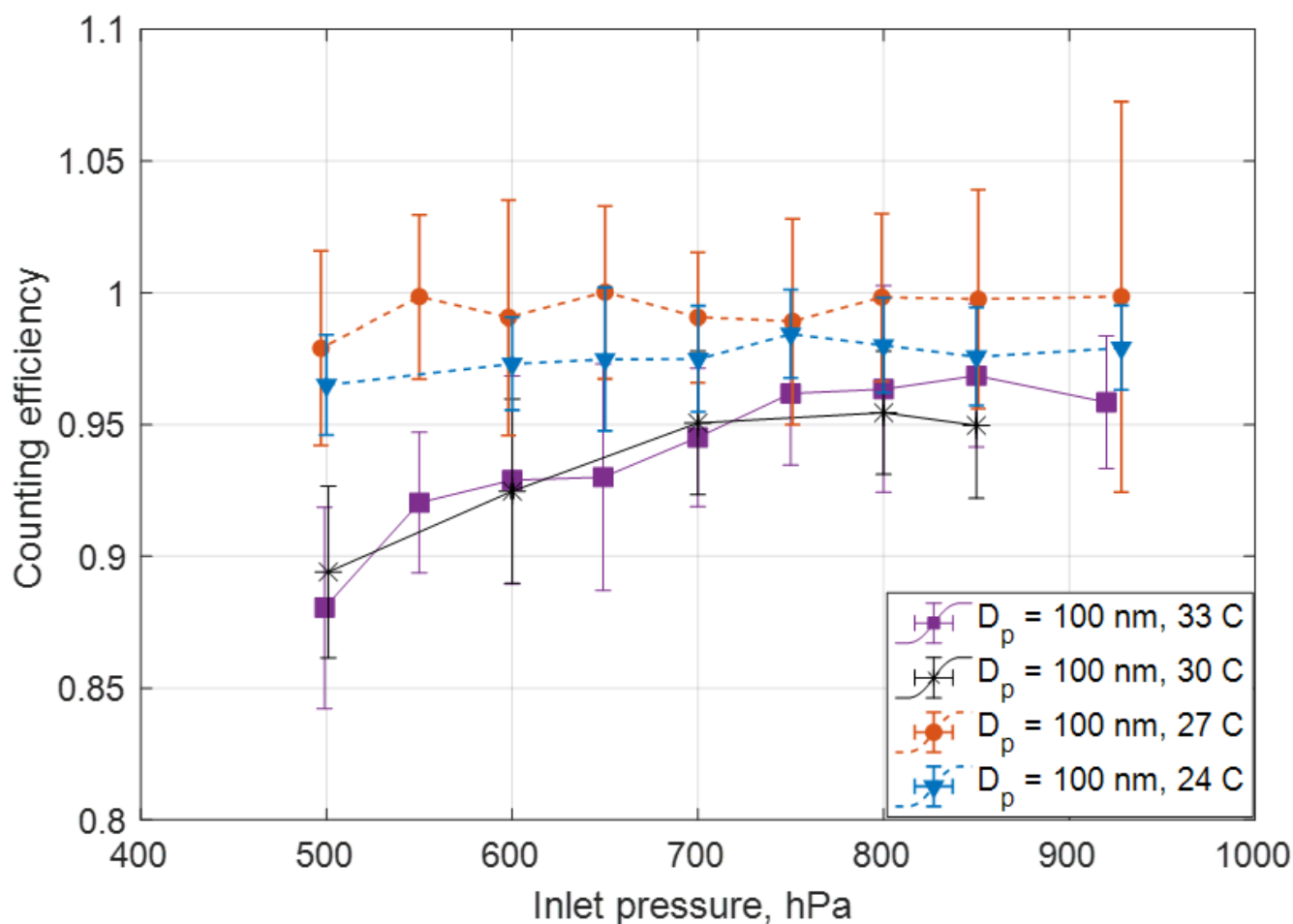
Fig. 6, CPC 3789 counting efficiency as a function of the inlet operation pressure at four conditioner temperatures of T_{\text{cond}} = 24, 27, 30, 33 °C ( T_{\text{ini}}=59^\circ\text{C} , T_{\text{mod}}=10^\circ\text{C} ).
