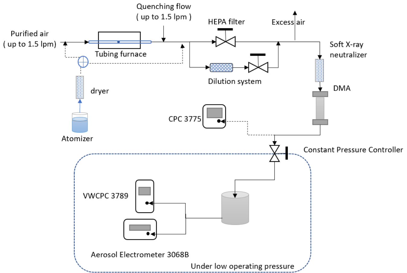
Figure 2. Schematic of the vWCPC sensors and flow system under the low-pressure testing.
