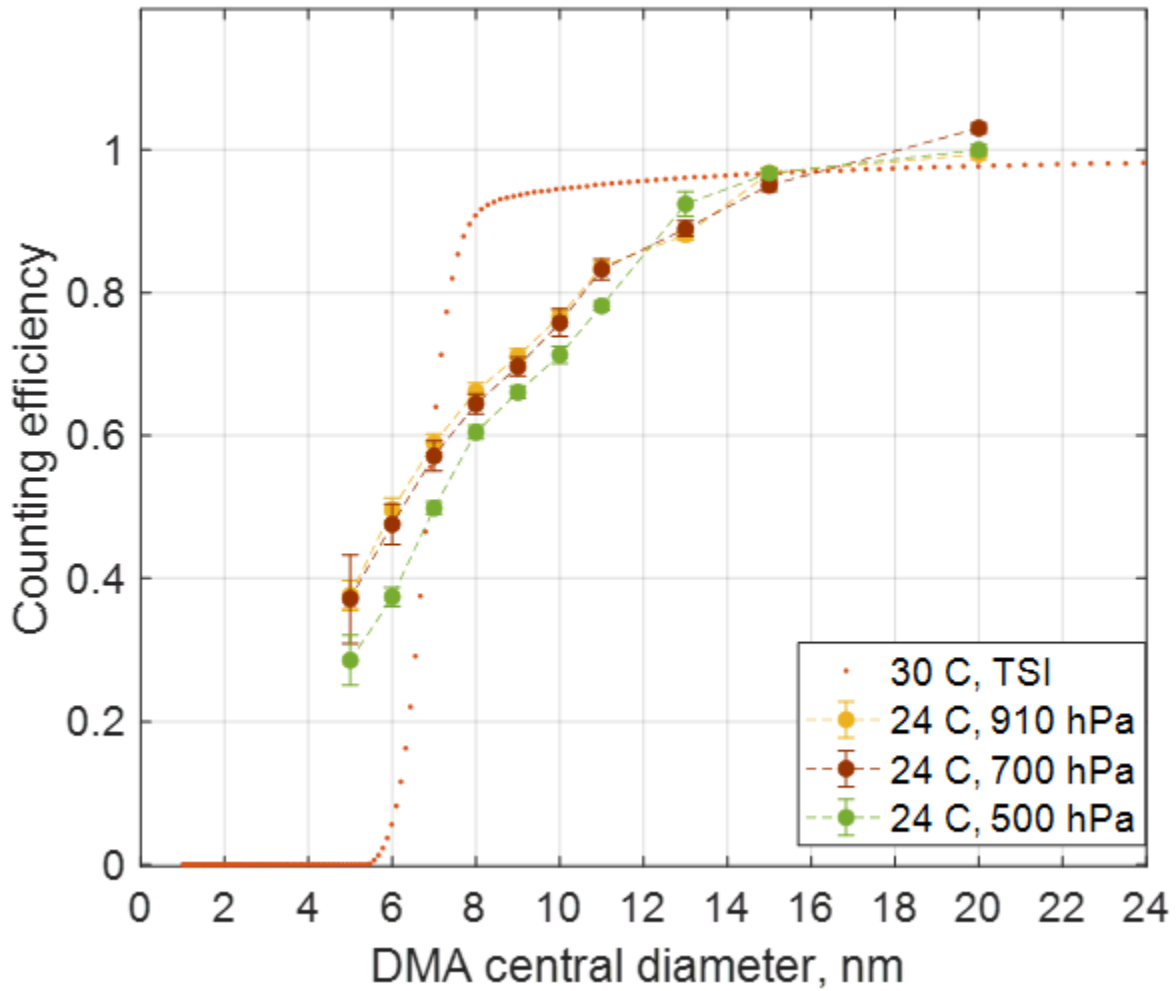
Fig. 9, CPC 3789 counting efficiency changes as a function of the different operating pressures (500, 700, and 910 hPa) using AS particles, when the initiator temperature is 59 °C, and the moderator temperature is 10 °C, at two different conditioner temperatures (a) Tcond = 24, (b) Tcond = 27 °C.
