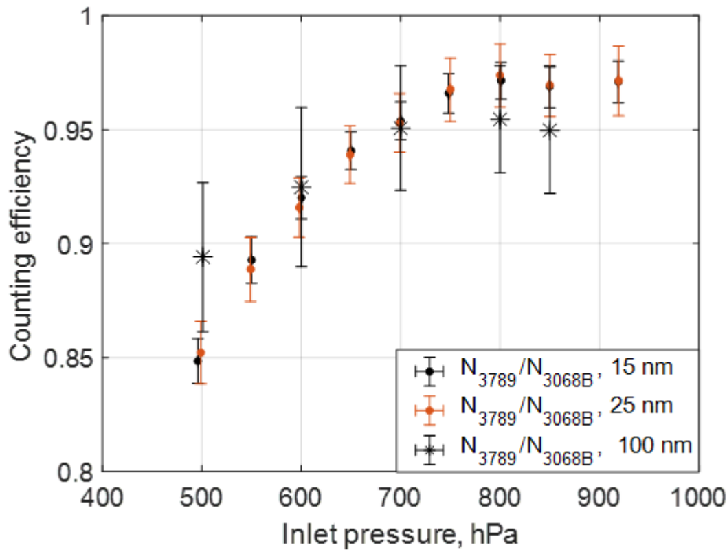
Fig. 3, CPC 3789 counting efficiency as a function of the inlet operation pressure at TSI standard conditions: T_{\text{cond}} = 30^\circ\text{C} , T_{\text{ini}} = 59^\circ\text{C} , and T_{\text{mod}} = 10^\circ\text{C} . N_{3789}/N_{3068B} is the total number concentration ratio between the vWCPC and the electrometer.
