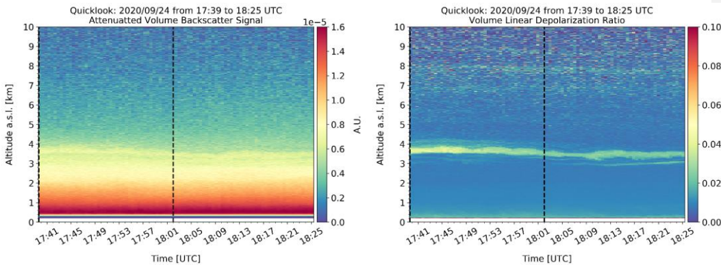
680 Figure 10: Height versus time plots of the attenuated volume backscatter signal from linear emission and the volume linear depolarisation ratio at 355 nm over Athens, measured by eVe lidar on 24 September 2020 from 17:39 to 18:25 UTC. The raw temporal and vertical resolution are 30 s and 3.75 m, respectively, with vertical pointing of the system. The attenuated volume backscatter signal was calibrated using a calibration factor averaged inside the selected timeframe and calculated at 9.8 km within a 0.2 km window. The two back dashed lines enclose the selected timeframe for the optical products retrieval.
