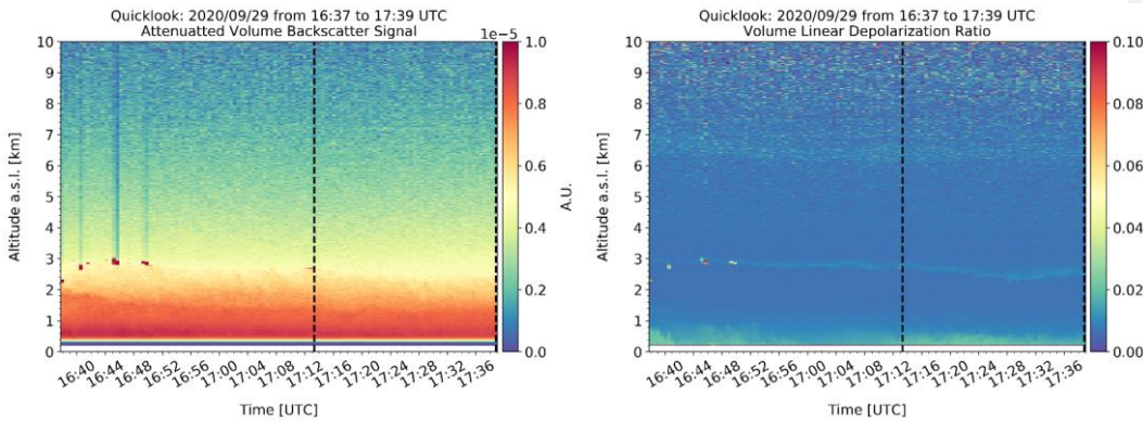
615 Figure 8: Height versus time plots of the attenuated volume backscatter signal from linear emission and the volume linear depolarisation ratio at 355 nm over Athens, measured by eVe lidar on 29 September 2020 from 16:37 to 17:39 UTC. The raw temporal and vertical resolution are 30 s and 3.75 m, respectively, with vertical pointing of the system. The attenuated volume backscatter signal was calibrated using a calibration factor averaged inside the selected timeframe and calculated at 3.8 km with a 0.3 km window. The two back dashed lines enclose the selected timeframe for the optical products retrieval.
