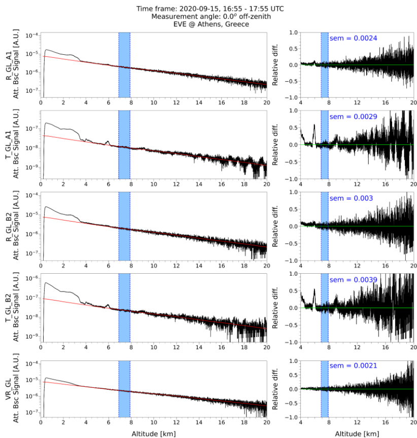
865 Figure B 1: The Rayleigh fit test from a one-hour nighttime measurement with vertical pointing of the lidar on 15 September 2020. In the first column, the elastic unsmoothed range-corrected glued signals from the Reflected (R_GL) and Transmitted (T_GL) channels of the A1 and B2 configurations and the inelastic unsmoothed range-corrected glued signal from the Raman channel (VR_GL) are normalised to the corresponding Rayleigh signals (red line) over the shaded blue region. In the second column, the relative difference of the normalised signals from the Rayleigh signals is presented along with the standard error of the mean (sem) 870 of the differences inside the reference region. The blue shaded region denotes the selected reference region for Rayleigh atmosphere ( 7.4 \pm 0.5 km).
