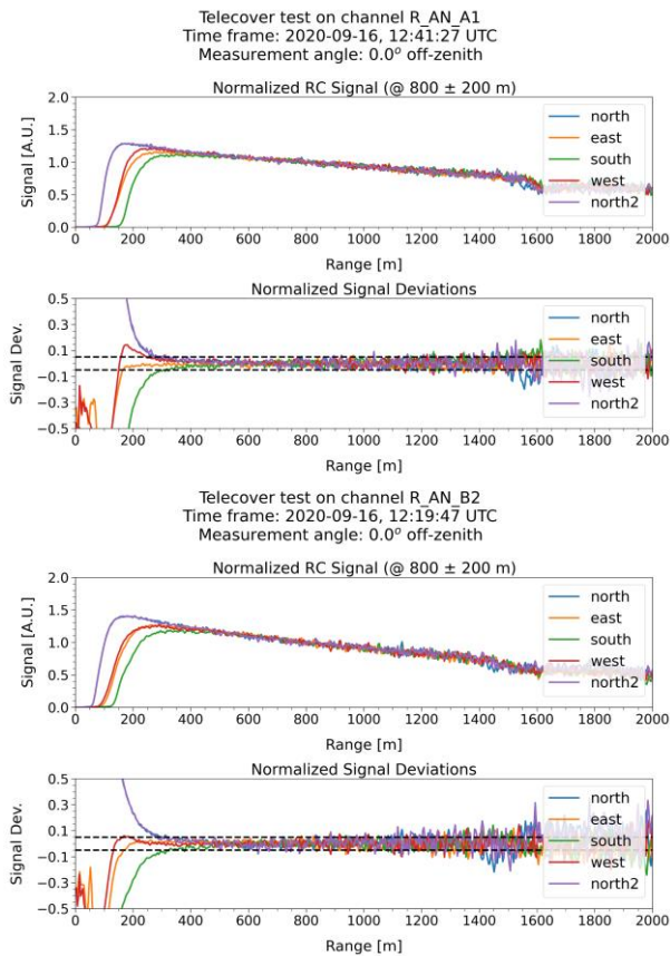
880 Figure B 2: The octant telecover test using the telecover signals from the Reflected (R) channels of the A1 and B2 configurations on 16 September 2020. The signals are unsmoothed range-corrected analogue signals normalised at 800 m with a window of 400 m
