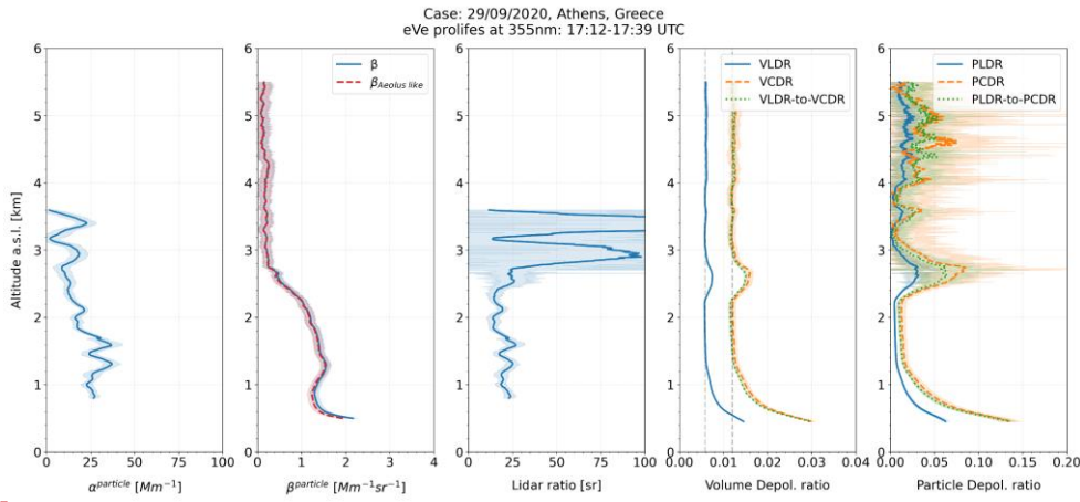
Figure 9: Profiles of the particle extinction coefficient, the particle backscatter coefficient, the lidar ratio, the volume depolarisation ratios and the particle depolarisation ratios (from left to right) at 355 nm for the timeframe 17:12 to 17:39 UTC on 29 September 2020. The ‘Aeolus like’ particle backscatter coefficient ( \beta_{Aeolus\ like} ; dashed red line) and the particle backscatter coefficient ( \beta ; solid blue line) were both retrieved from the circularly polarised signals of eVe lidar using the Raman inversion method where the reference height for Rayleigh atmosphere was selected at 10.3 km with a 0.3 km window. The VLDR and PLDR profiles are presented in blue solid lines, the VCDR and PCDR profiles are presented in orange dashed lines, while the VLDR-to-VCDR and PLDR-to-PCDR profiles are presented in green dotted lines. The corresponding mLDR and mCDR values (dashed grey lines) that are expected to be measured by the lidar are also provided in the volume depolarisation ratio subplot. Shaded regions denote statistical 1\sigma uncertainty.
