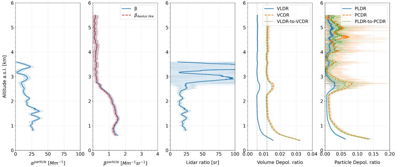
600 Figure 9: Profiles of the particle extinction coefficient, the particle backscatter coefficient, the lidar ratio, the volume depolarisation ratios and the particle depolarisation ratios (from left to right) at 355 nm for the timeframe 17:12 to 17:39 UTC on 29 September 2020. The ‘Aeolus like’ particle backscatter coefficient ( \beta_{Aeolus\ like} ; dashed red line) and the particle backscatter coefficient ( \beta ; solid blue line) were both retrieved from the circularly polarised signals of eVe lidar using the Raman inversion method where the reference height for Rayleigh atmosphere was selected at 10.3 km with a 0.3 km window. The VLDR and PLDR profiles are presented in blue solid lines, the VCDR and PCDR profiles are presented in orange dashed lines, while the VLDR-to-VCDR and PLDR-to-PCDR profiles are presented in green dotted lines. The corresponding mLDR and mCDR values (dashed grey lines) that are expected to be measured by the lidar are also provided in the volume depolarisation ratio subplot. Shaded regions denote statistical 1\sigma uncertainty. 605
