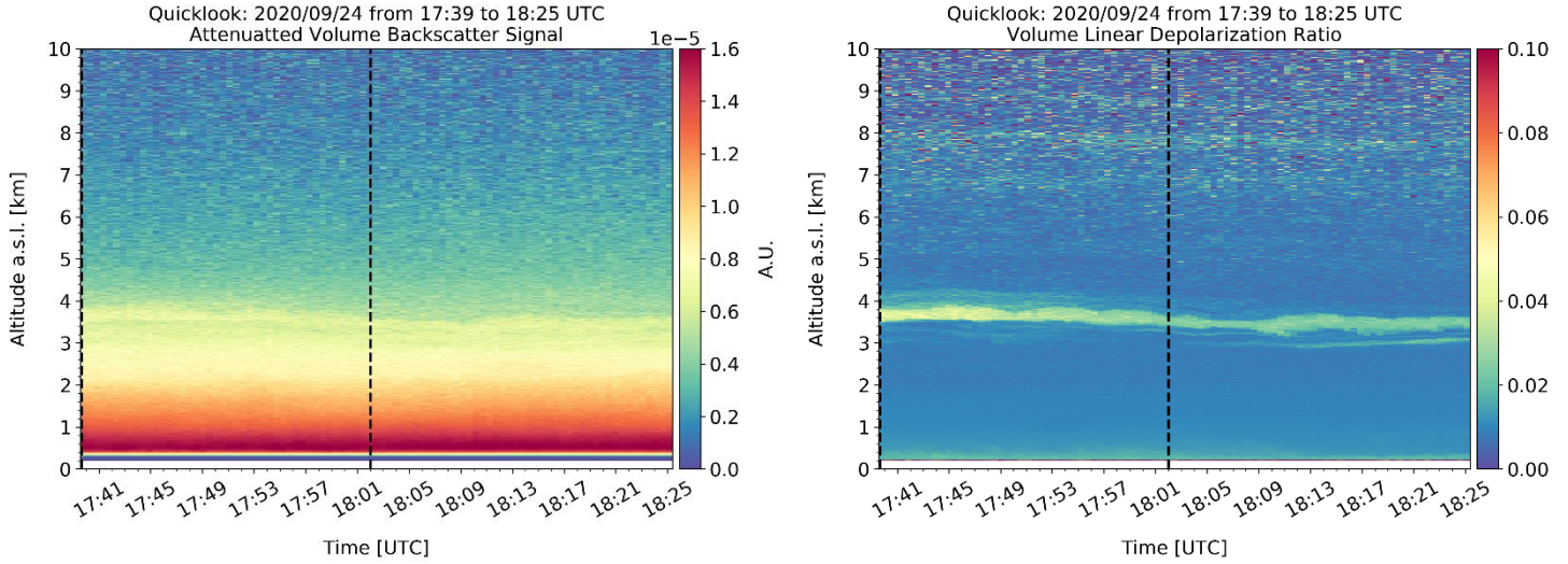
625 Figure 10: Height versus time plots of the attenuated volume backscatter signal from linear emission and the volume linear depolarisation ratio at 355 nm over Athens, measured by eVe lidar on 24 September 2020 from 17:39 to 18:25 UTC. The raw temporal and vertical resolution are 30 s and 3.75 m, respectively, with vertical pointing of the system. The attenuated volume backscatter signal was calibrated using a calibration factor averaged inside the selected timeframe and calculated at 9.8 km within a 0.2 km window. The two back dashed lines enclose the selected timeframe for the optical products retrieval.
