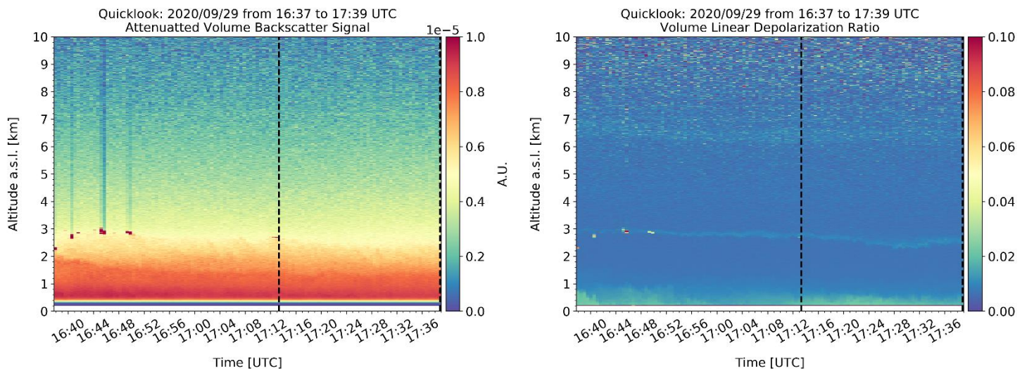
575 Figure 8: Height versus time plots of the attenuated volume backscatter signal from linear emission and the volume linear depolarisation ratio at 355 nm over Athens, measured by eVe lidar on 29 September 2020 from 16:37 to 17:39 UTC. The raw temporal and vertical resolution are 30 s and 3.75 m, respectively, with vertical pointing of the system. The attenuated volume backscatter signal was calibrated using a calibration factor averaged inside the selected timeframe and calculated at 3.8 km with a 0.3 km window. The two back dashed lines enclose the selected timeframe for the optical products retrieval.
