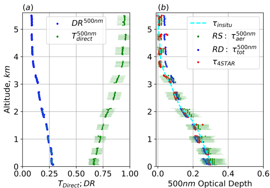
Figure 5: ORACLES spiral on 20181003. (a) DR^{500nm}_{mea} and T^{500nm} with the associated measurement uncertainty shown by the shading. (b) \tau_{aer} profiles derived from RS, 4STAR, in situ, and RD.
