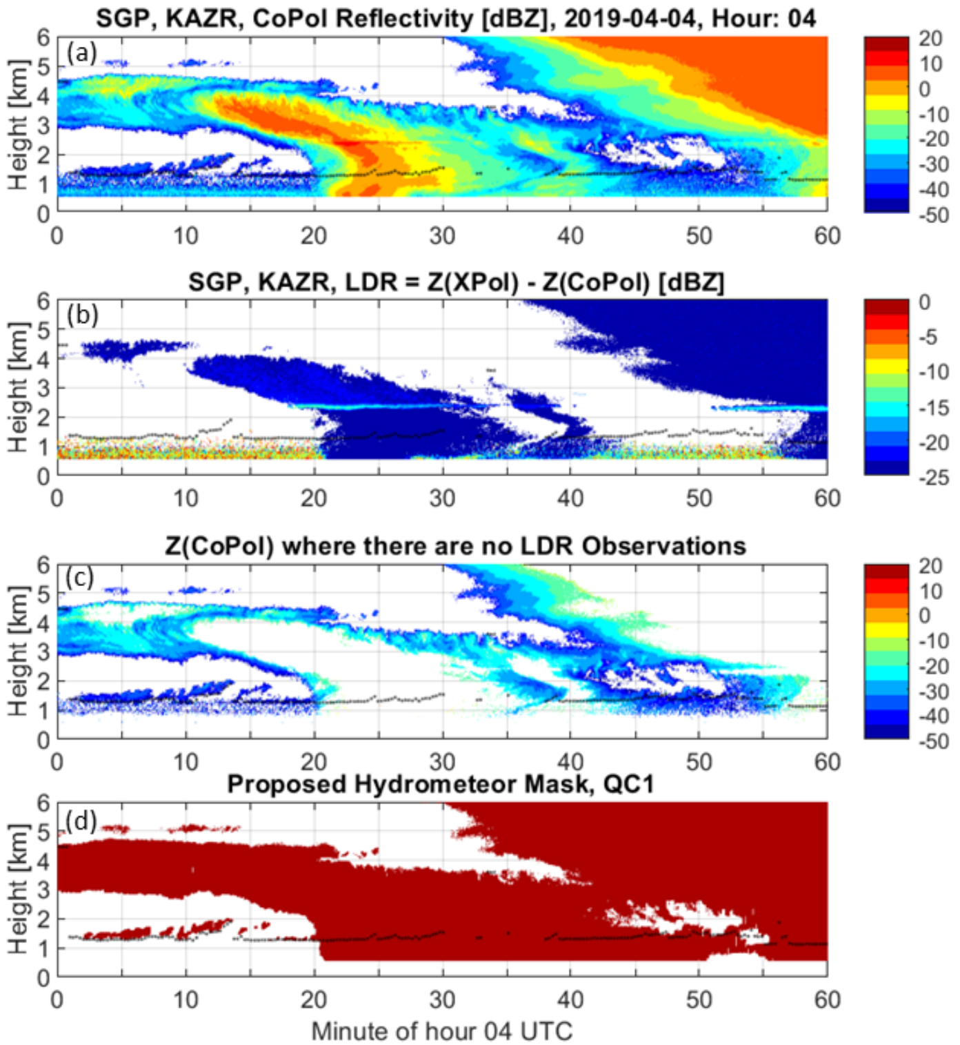
Figure 4: Moments calculated from raw spectra and retrieved hydrometeor QC1 mask for hour 4 UTC on 4-April-2019. (a) CoPol reflectivity [dBZ]. (b) Linear depolarization ration (LDR) [dB]. (c) CoPol reflectivity [dBZ] at pixels that do not have an LDR measurement. (d) Retrieved hydrometeor QC1 mask. Black symbols in both panels are ceilometer derived cloud base.
