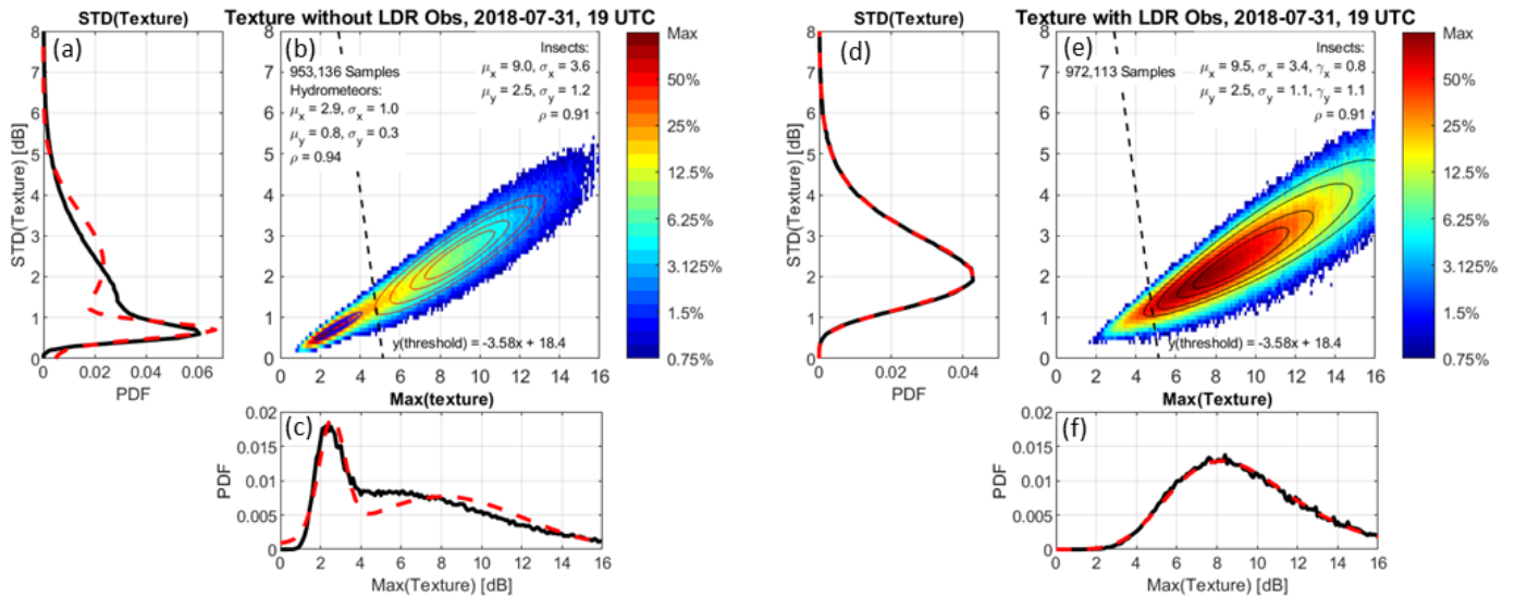
Figure 7: 1D and 2D distributions of texture statistics from hour 19 UTC on 31-July-2018. There are 953,136 spectra regions used in these distributions. (a) 1D PDF of STD(Texture). Black line is observations and red dashed line is fit to two Gaussian distributions. (b) Colors are observed 2D distribution of STD(Texture) vs. Max(Texture). Colors represent drop from pixel with most occurrences. Blue and red contours are 2D Gaussian fits to hydrometeors (blue) and insects (red). Contours represent 90%, 75%, 63%, and 50% occurrence. Gaussian fit parameters are displayed in panel. Threshold between hydrometeor and insect indicated by dashed black line at \max(\text{texture}) = 4.5 . (c) 1D PDF of Max(Texture). Black line is observations and red line is fit to two Gaussian distributions.
