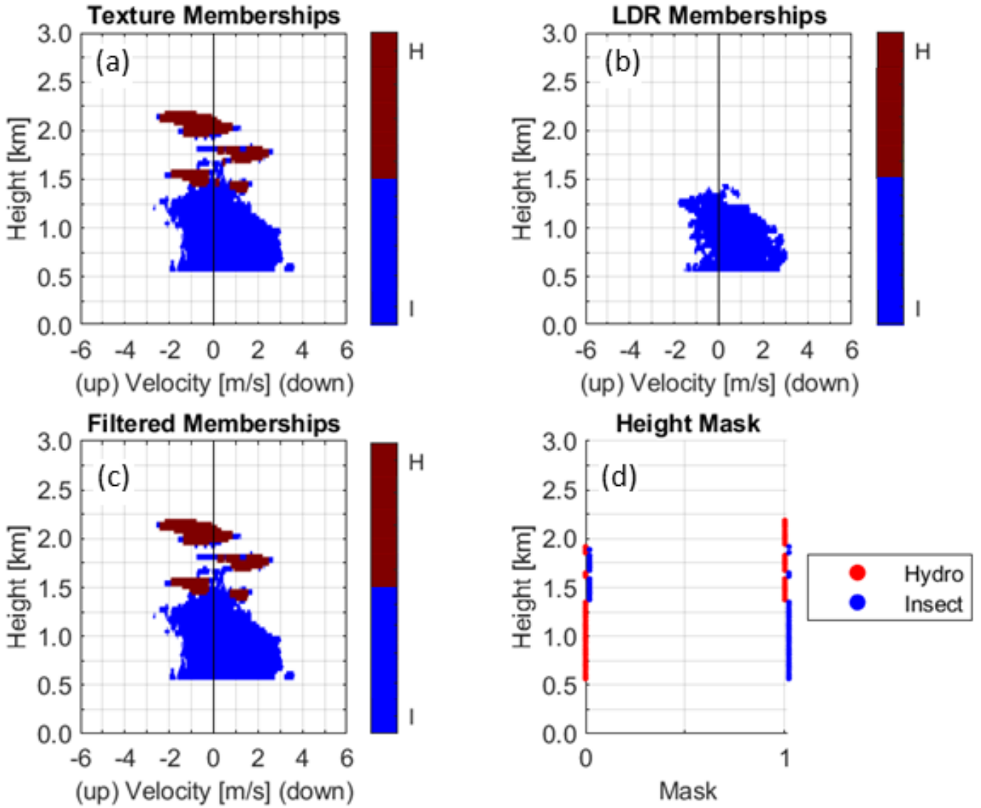
Figure 8: Spectral memberships and binary mask for profile at 19:19:02 UTC on 31-July-2018. Red color indicates hydrometeor membership and blue color represents insect membership (a) Texture algorithm spectral membership. (b) LDR algorithm spectral membership. (c) Filtered spectral membership. (d) Binary hydrometeor and insect mask.
