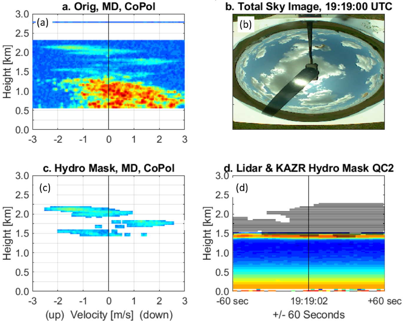
Figure 14: Measurement and retrievals near profile 19:19:02 UTC on 31 July 2018. (a) Doppler velocity power spectra. (b) Total Sky Imager (TSI) photo. (c) Doppler velocity power spectra screened by spectral hydrometeor mask. (d) Doppler lidar attenuated backscattered power for +/- 60 s of profile 19:19:02 UTC. Black lines indicate hydrometeor QC2 mask for +/- 60 s of profile 19:19:02 UTC.
