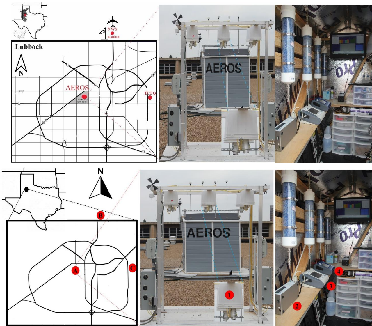
125 Figure 1. Location of AEROS (A) in the South High Plains of West Texas with locations of meteorological station (B) and TCEQ PM 2.5 station (C). The photos show the filter sampler unit with Harvard Impactor (HI:1) units and the aerosol measurements unit (outside and inside view with dryers and instruments 2-Grimm 11-D, 3-OPS, and 4-DustTrak).
