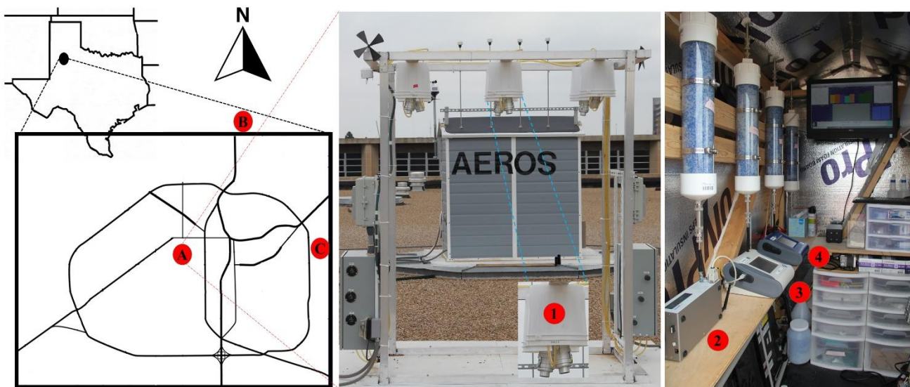
Figure 1. Location of AEROS (A) in the South High Plains of West Texas with locations of meteorological station (B) and 125 TCEQ PM 2.5 station (C). The photos show the filter sampler unit with Harvard Impactor (HI;1) units and the aerosol measurements unit (outside and inside view with dryers and instruments 2-Grimm 11-D, 3-OPS, and 4-DustTrak).
