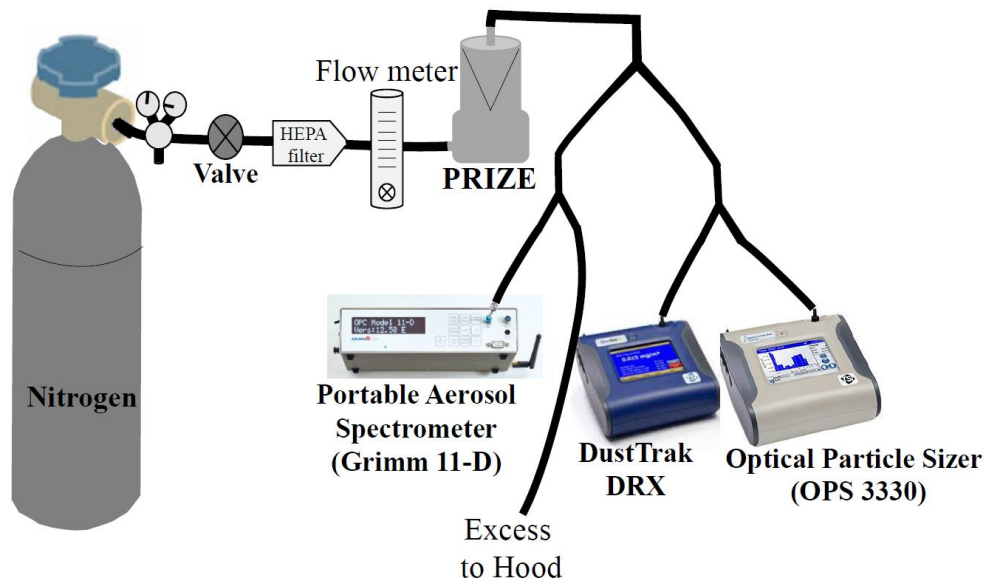
Figure 2. Experimental setup: Arizona Test Dust (ATD) particles were generated using PRinted FluidIZed bed gEnerator- 3D 235 dust generator (PRIZE) and measured by the various instruments (DustTrak, OPS, and Grimm 11-D).
