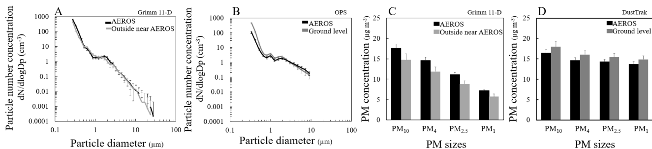
Figure 6. Comparison of measurements taken in the AEROS shed with measurements taken on the ground level or the rooftop floor outside the AEROS shed. (A) Particle size distribution (optical diameter) measured by the Grimm 11-D unit in the AEROS shed (black) and outside on the rooftop floor (light gray). (B) Particle size distribution (optical diameter) measured by the OPS in AEROS (black) and on the ground floor (dark gray). (C) PM concentration at various sizes as measured by the Grimm 11-D unit in AEROS (black) and outside AEROS on the rooftop floor (gray). (D) PM concentration at various sizes as measured by DustTrak in AEROS (black) and on the ground floor (dark gray). Error bars represent SD values of the measured period.
