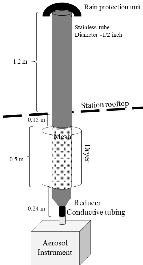
Figure S1. Schematic of station inlet.
