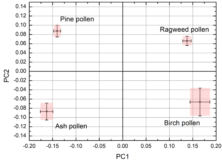
Figure 6: Projection of the ten f_{ij} scattering matrix elements (five per wavelength) for each pollen on the new ( PC_1, PC_2 )-orthogonal basis using principal component analysis. Error bars have been evaluated by propagating the uncertainties on each f_{ij}^\lambda scattering matrix element. Coloured regions correspond to the range of ( PC_1, PC_2 ) where the pollen taxon can be unequivocally identified among our set of four pollen.
