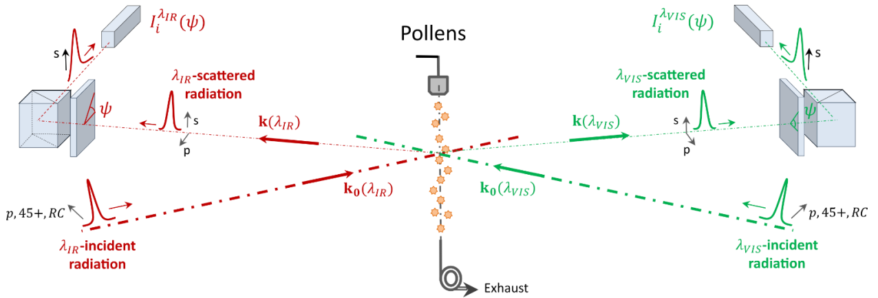
165 Figure 2: Scheme of the laboratory experimental set-up of the (\lambda_{VIS}, \lambda_{IR}) polarimeter from (Cholleton et al., 2020). The 177.5^\circ scattering angle has been exaggerated to ease the reading. \mathbf{k}_0(\lambda) and \mathbf{k}(\lambda) respectively stand for the incident and scattered wavevectors at wavelength \lambda . Pollen grains are embedded in laboratory ambient air as described Section 2.5. \psi is the angle between the fast axis of the quarter-wave plate (QWP) and the scattering plane.
