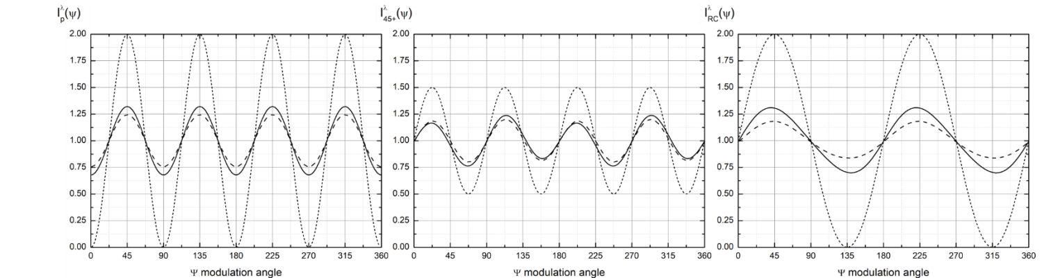
Figure 3: Numerical simulation of the detected scattered light intensity I_i^\lambda(\psi) as a function of the \psi -angle of the analyser for the three considered case studies of pollen taxa : Taxon 1 (dotted lines), Taxon 2 (solid lines), Taxon 3 (dashed lines) at the three successive incident polarization states ( i = (p), (45^\circ), (RC) ) from left to right. Each curve is normalized to unity (i.e. I_0^\lambda \times a_i^\lambda = 1 ) so that any change in the scattered light intensity be due to polarimetric considerations.
