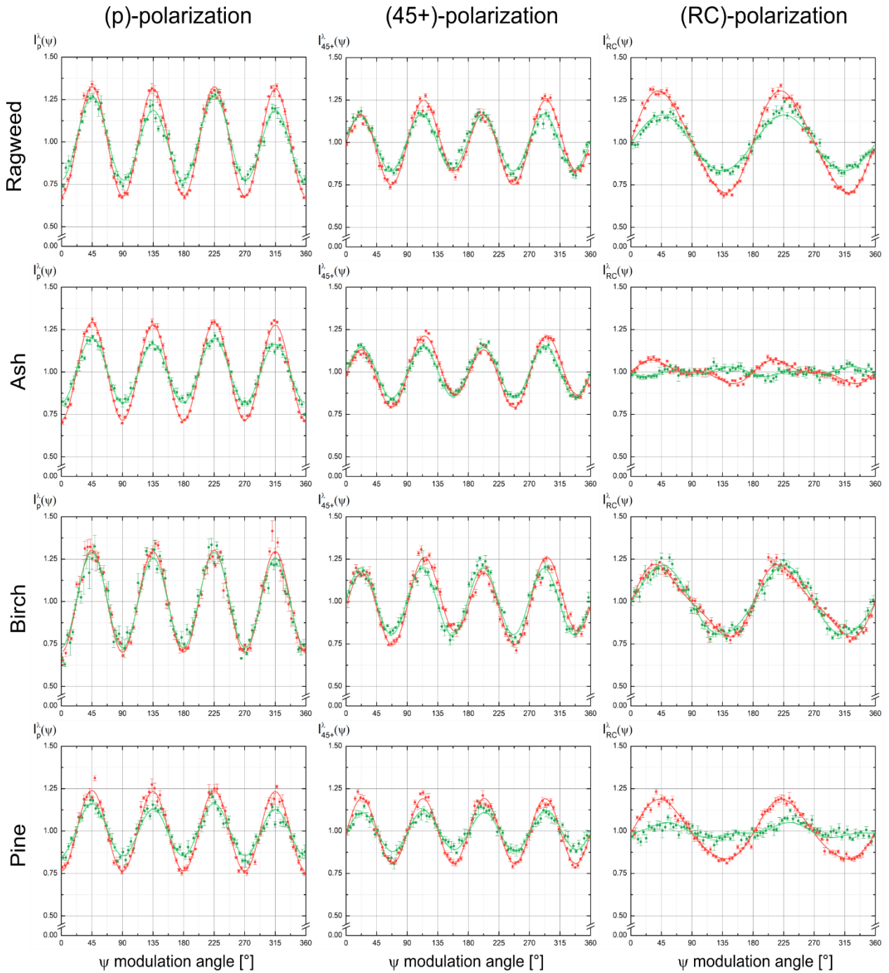
295 Figure 4: Detected scattered light intensity by ragweed, ash, birch and pine pollen as a function of the of the \psi -angle of the analyser for the three successive incident polarization states (p), (45+) and (RC) at wavelength \lambda_{VIS} (in green) and wavelength \lambda_{IR} (in red). The detected light intensity is normalized so that \mathbf{a}_i \times \mathbf{I}_0^\lambda = \mathbf{1} , as detailed Section 3.3. A break has been inserted to ease the reading. Each measurement data point is obtained by repeating 400 lasers shots and the uncertainty is calculated by following the methodology described in Section 3.4.
