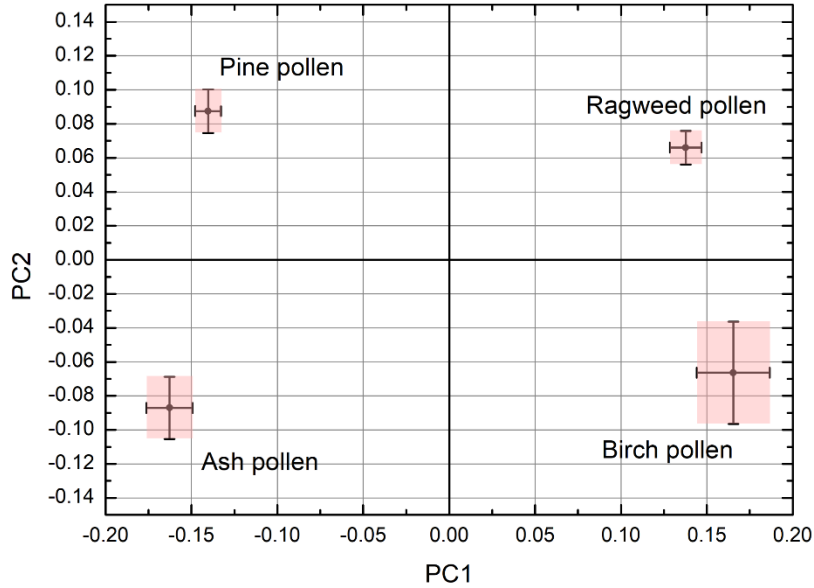
Figure 6: Projection of the ten f_{ij}^\lambda scattering matrix elements (five per wavelength) for each pollen on the new ( PC_1, PC_2 )-orthogonal basis using principal component analysis. Error bars have been evaluated by propagating the uncertainties on each f_{ij}^\lambda scattering matrix element. Coloured regions correspond to the range of ( PC_1, PC_2 ) where the pollen taxon can be unequivocally identified among our set of four pollen.
