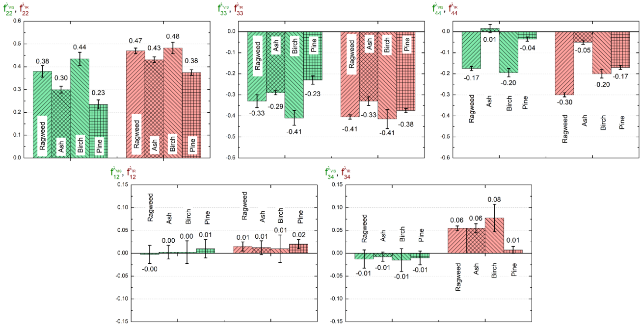
300 Figure 5: Retrieved scattering matrix elements of ragweed, ash, birch and pine at 177.5^\circ scattering angle at wavelengths \lambda_{VIS} and \lambda_{IR} , with corresponding uncertainties evaluated by applying the methodology presented in Section 3. For each pollen taxon, the evaluation of the scattering matrix has been repeated with different samples: each evaluated scattering matrix lies within presented error bars.
