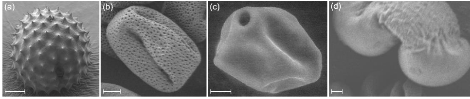
125 Figure 1 : Scanning electron microscopy (SEM) images of the studied pollen taken at iLM: (a) ragweed ( Ambrosia artemisiifolia ), (b) ash ( Fraxinus americana ), (c) birch ( Betula pendula ), (d) pine ( Pinus strobus ). The scale bar is 5 \mu\text{m} on all pictures. Pollen grains were suspended in ambient air and deposited on an adhesive substrate for SEM observations.
