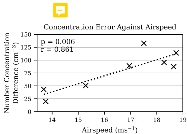
Figure 14. A correlation plot of the absolute difference in measured number concentration between the FMI-Talon and Static UCASS units, and airspeed, for the 28 th of September. The linear regression line and ‘p’ value are shown.
