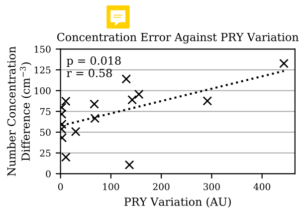
Figure 15. A correlation plot of the absolute difference in measured number concentration between the FMI-Talon and Static UCASS units, and PRY Variation, for the whole campaign. The linear regression line and ‘p’ value are shown.
