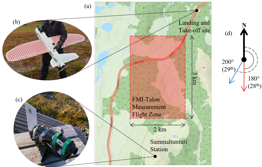
Figure 7. A series of illustrations designed to give context to the measurement campaign. Figure 7a shows a map of the area including Sammaltunturi station, the UAV landing site, and the flight operations zone in the red square; b shows the UCASS mounted to the FMI-Talon; c is an image of the UCASS – wind-vane system mounted to the station; and d shows the wind directions, measured by Sammaltunturi station, on the 28 th and 29 th with red and blue arrows respectively.
