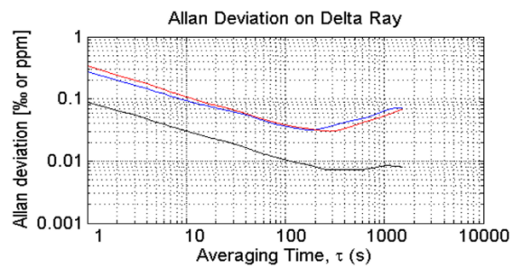
1075 Figure 3: Allan deviation determined in QC-1: blue = \delta^{13}\text{C} , red = \delta^{18}\text{O} , black = \text{CO}_2 , determined during the 2015 campaign.
