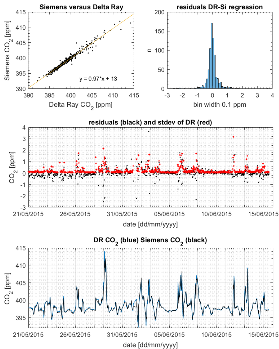
Figure 12: Top left: slope and scatter of the regression Siemens (Si) versus Delta Ray (DR). Top right: histogram of residuals (top right). Middle: residuals (black) and 1\sigma standard deviation of the DR measurements (red). Bottom: CO 2 mole fractions from DR (blue) and Siemens (black).
