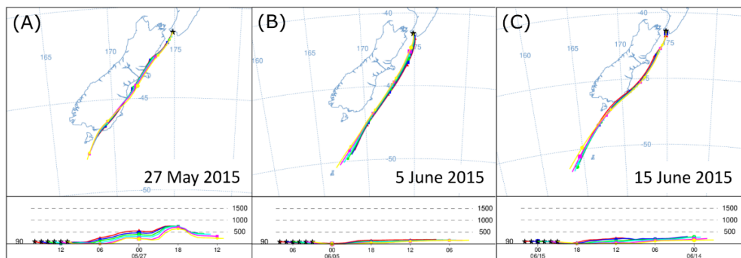
1150 | Figure 7: HYSPLIT back trajectories (24 h) for the air measured during S1, S2 and S3, with a 1 h interval between displayed trajectories. The selected timing is consistent with the final 6 h of each event displayed in Figure 16 with the lowest Radon radon counts.
