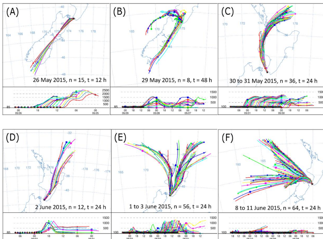
1195 Figure 12: HYSPLIT back trajectories from six events in the Delta Ray time series. Each panel shows the history of air that was measured at the stated date. Intervals between trajectories are 1 h, n indicates the number of trajectories in the panel, t represents the trajectory length in hours.
