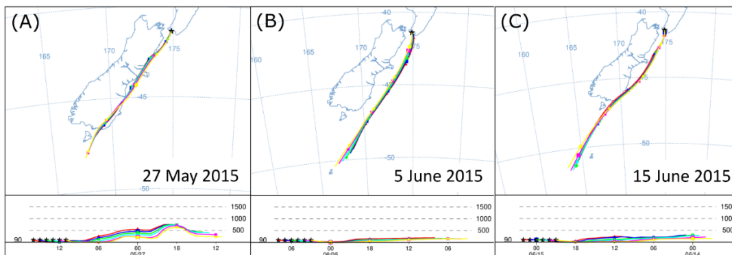
1210 Figure 13: HYSPLIT back trajectories (24 h) for the air measured during S1, S2 and S3, with a 1 h interval between displayed trajectories. The selected timing is consistent with the final 6 h of each event displayed in Figure 17 with the lowest Radon counts.
