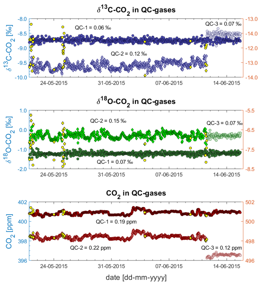
Figure 6: QC gas data as measured against Ref-1 during deployment at BHD, \delta^{13}\text{C-CO}_2 (top), \delta^{18}\text{O-CO}_2 (middle) and \text{CO}_2 mole fractions (bottom). QC-1 and QC-3 on left y-axes, QC-2 on right y-axes.
