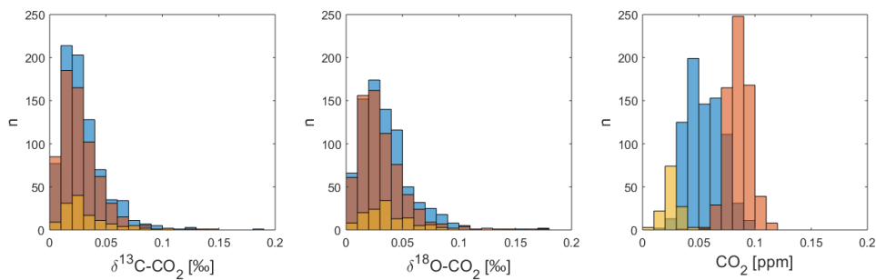
Figure 7: Internal reproducibility as the standard deviation ( 1\sigma ) of the QC gas block averages in each sequence for \delta^{13}\text{C-CO}_2 (left), \delta^{18}\text{O-CO}_2 (middle) and \text{CO}_2 mole fractions (right), outliers excluded. QC-1 in blue, QC-2 in red and QC-3 in yellow.
