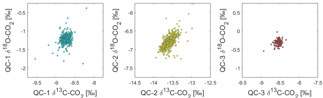
Figure 8: Correlation of \delta^{13}\text{C-CO}_2 and \delta^{18}\text{O-CO}_2 values in QC-1 (left), QC-2 (middle) and QC-3 (right) before outlier removal and correction for QC-1.
