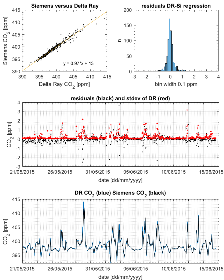
1175 Figure 10: Top left: slope and scatter of the regression Siemens (Si) versus Delta Ray (DR). Top right: histogram of residuals (top right). Middle: residuals (black) and 1σ standard deviation of the DR measurements (red). Bottom: CO 2 mole fractions from DR (blue) and Siemens (black).
