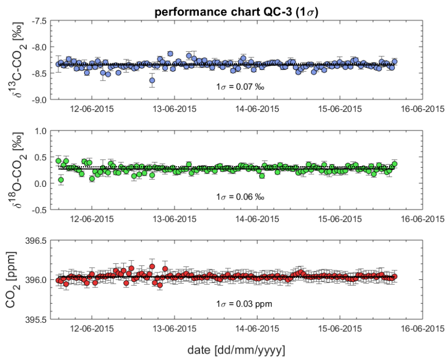
Figure 9: Sequence averages for processed \delta^{13}\text{C-CO}_2 (top), \delta^{18}\text{O-CO}_2 (middle) and \text{CO}_2 (bottom) in QC-3. The standard deviation ( 1\sigma ) is a measure of the achievable analytical precision.
