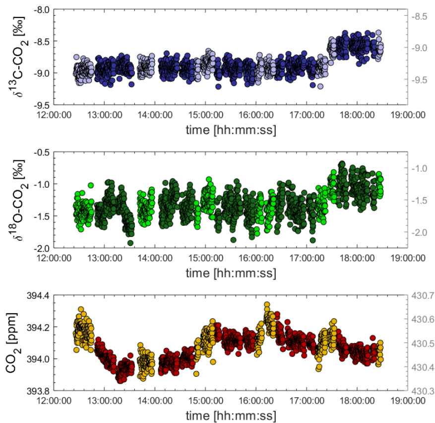
Figure 4: Sudden and synchronous shift in both \delta^{13}\text{C-CO}_2 (top) and \delta^{18}\text{O-CO}_2 (middle) affecting the measurement of two QC gases during laboratory tests. Shifts in isotope traces are not reflected in \text{CO}_2 mole fractions (bottom). Causes of the isotope shifts are unknown.
