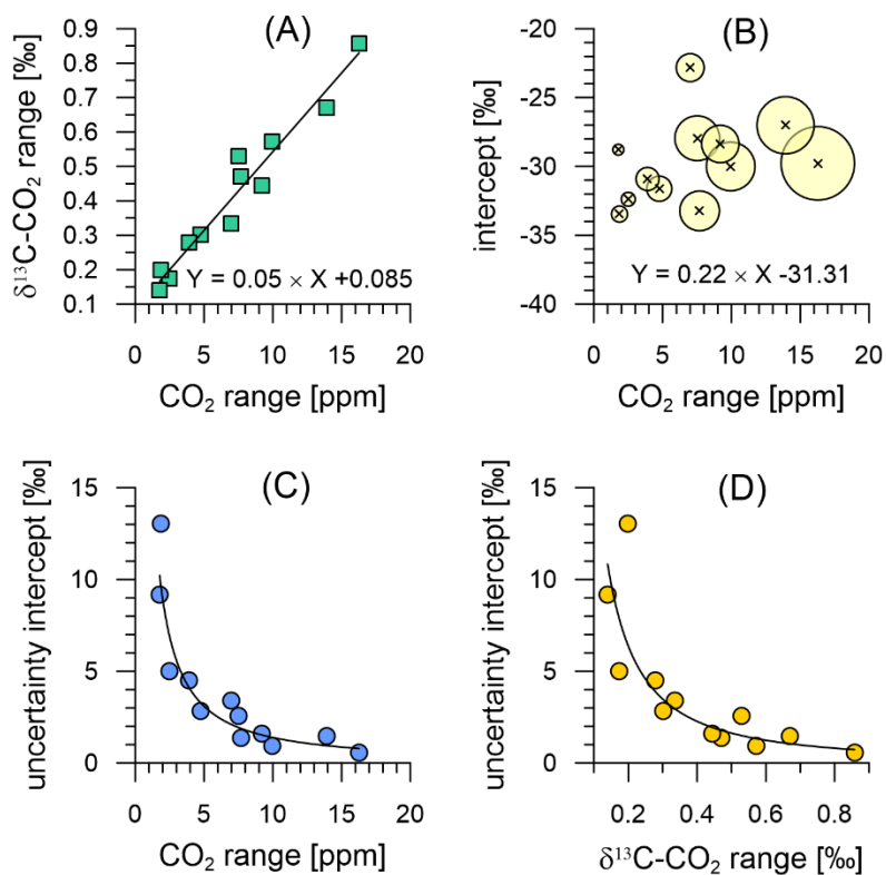
Figure 15: Relationship between the variations in \text{CO}_2 and \delta^{13}\text{C-CO}_2 of the twelve events used for KPA (A), as well as their intercept as function of the covered \text{CO}_2 range (B). The bubble size in (B) scales with the range in \delta^{13}\text{C-CO}_2 covered within the KPA event. Uncertainty of the intercept (standard error) as function of the range in \text{CO}_2 (C) and \delta^{13}\text{C-CO}_2 (D).
