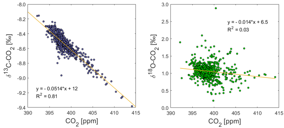
Figure 14: Correlation between CO 2 and δ 13 C-CO 2 (left) and δ 18 O-CO 2 (right) in air (n = 791).
