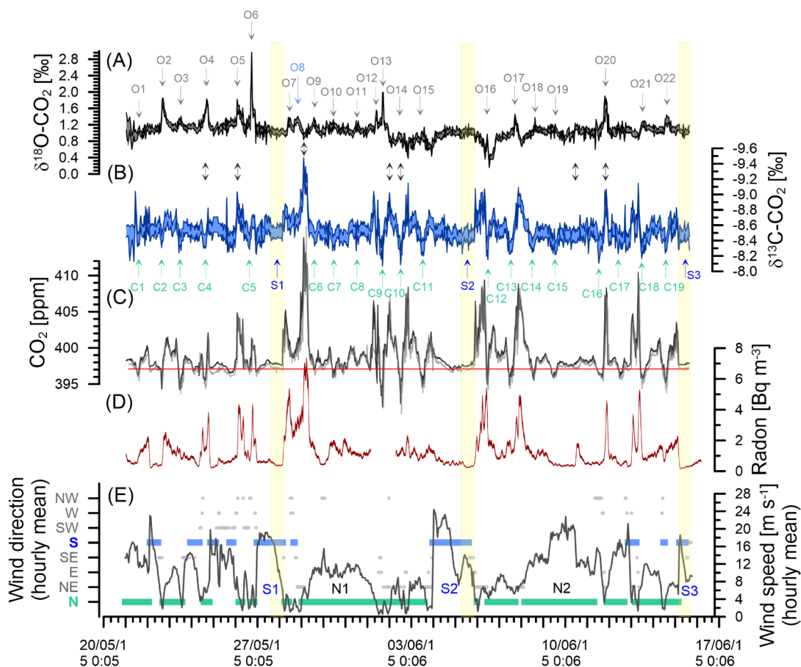
Figure 11: Observations during the deployment at BHD. Delta Ray time series of \delta^{18}\text{O-CO}_2 (A) and \delta^{13}\text{C-CO}_2 with inverted y-axis (B). \text{CO}_2 mole fractions measured with Delta Ray (black) and Siemens (grey) with average of the Siemens analyser for baseline \text{CO}_2 measured during S2 indicated in red (C). Coloured shading in (A), (B) and (C) indicates the standard deviation of the measurement averages of the Delta Ray measurements. Events in the \delta^{18}\text{O-CO}_2 and \delta^{13}\text{C-CO}_2 time series are numbered from O1 to O22 and C1 to C19, respectively. (D) shows the Radon time series and (E) hourly averages of meteorological data. Southerly and northerly wind events are highlighted in blue and green, respectively. Wind speed is displayed by the black line. The yellow boxes highlight the most stable periods of the three significant southerly events S1, S2 and S3.
