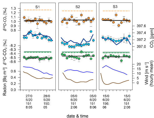
1280 Figure 17: Data from southerly events S1 (left), S2 (middle) and S3 (right). Radon is shown in brown lines, mean hourly wind speed 1285 in blue lines. Green, blue, and orange filled circles show average Delta Ray values for \delta^{13}\text{C-CO}_2 , \text{CO}_2 mole fractions and \delta^{18}\text{O-CO}_2 , respectively. Error bars indicating the standard deviation ( 1\sigma ). Flat black lines indicate the event averages of the Delta Ray values for \delta^{13}\text{C-CO}_2 and \delta^{18}\text{O-CO}_2 . The dark green line shows the interpolated \delta^{13}\text{C-CO}_2 value measured in flask samples before and after the test campaign, while dashed lines represent the interpolated values from \delta^{13}\text{C-CO}_2 and \delta^{18}\text{O-CO}_2 observations at Cape Grim observatory. The dark blue line shows the \text{CO}_2 mole fraction values as interpolated from 5 min averages of the Siemens analyser at BHD.
