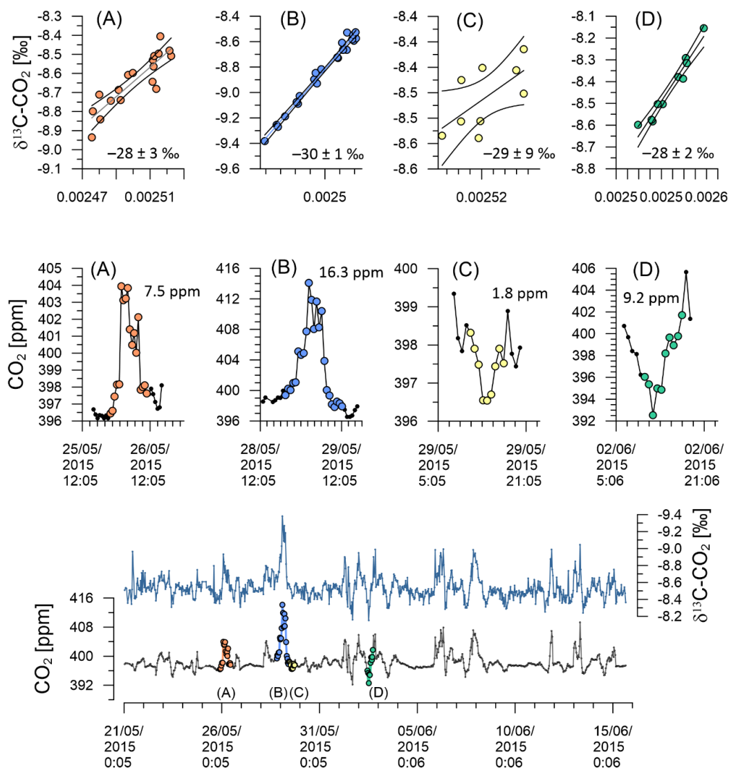
Figure 16: CO 2 and δ 13 C-CO 2 time series with selected events (A-D) shown in colours on the CO 2 time series (bottom panel). CO 2 variation of events A-D (middle panel). KPA with 95 % confidence interval and standard error for the intercept of A-D (top panel).
