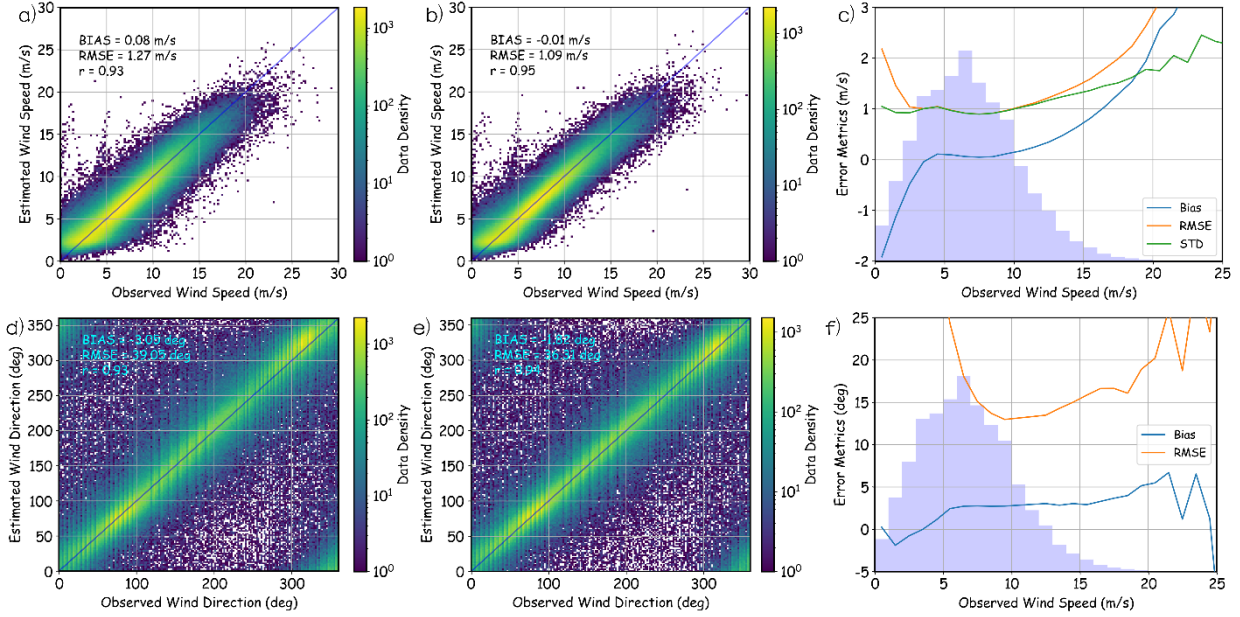
115 Figure 2. (a-c) Comparison between wind speeds measured by buoys and those estimated by wave spectra. (a) Scatter plot of collocated DNN-estimated wind speed and direct-measured wind speed. (b) The same as (a), but the spectra were used to estimate the wind speed 40 minutes ago. (c) The bias, STD, and RMSE of the DNN-estimated wind speed one hour ago as a function of direct-measured wind speed. The blue shadow indicates the empirical distribution function of direct-measured wind speed. (d-f) The same as (a-c), but for wind directions. 120
