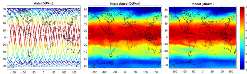
380 Figure 8. Left: ozone at limb satellite measurements at 10 hPa on 1 September 2018. Center: after interpolation. Right: corresponding adjusted SILAM ozone field at the same pressure level.
