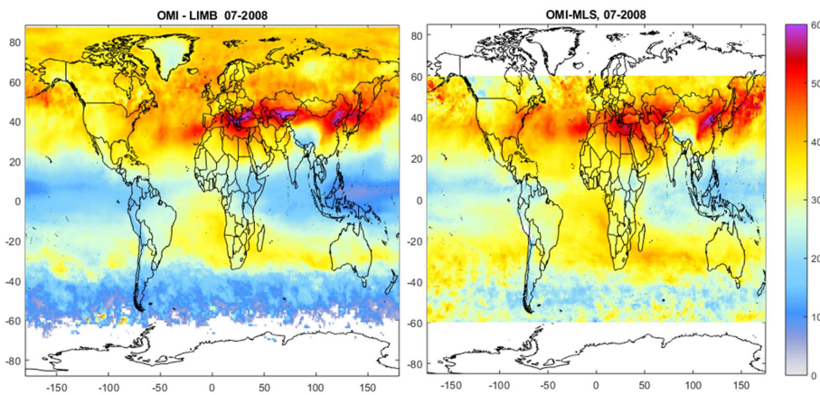
Figure 16. Left: SUNLIT tropospheric ozone column for July 2008 (OMI minus limb SOC); right: NASA OMI-MLS tropospheric ozone column.
