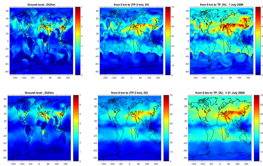
210 Figure 3. Simulations with SILAM for 1 July 2008 (top panels) and monthly mean for July 2008 (bottom panels). Left: ground level ozone, center: truncated tropospheric ozone column (from ground to the altitude 3 km lower than the tropopause, right: the full tropospheric ozone column (from ground to the tropopause).
