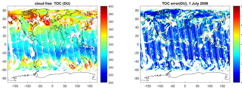
305 Figure 5. OMI Level 3 total ozone column data (left) and random uncertainty (right) for 1 July 2008.
