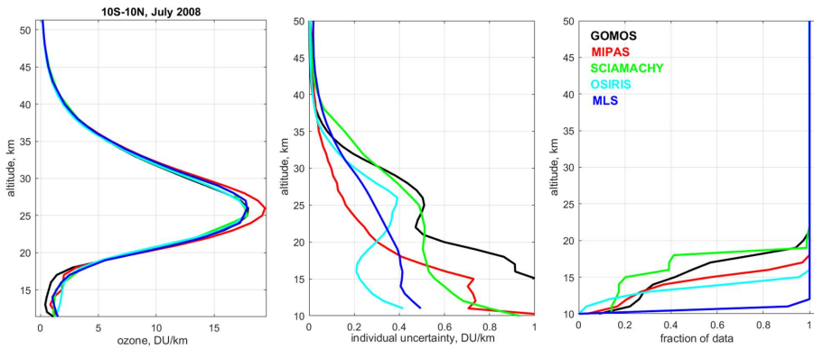
145 Figure 1. Left: mean ozone profiles at 10S-10N in July 2008. Center: uncertainty of individual ozone profiles, right: fraction of data (with respect to the data in the stratosphere).
