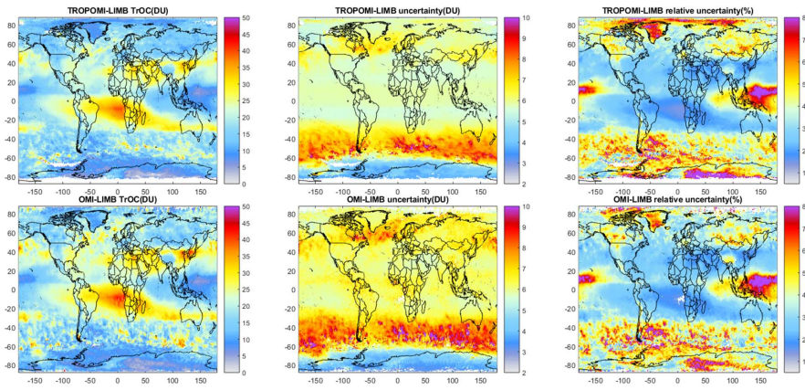
450 Figure 11. SUNLIT tropospheric ozone distributions (DU, color) for September 2018, from TROPOMI (top left) and OMI (bottom left). The stratospheric ozone column is estimated from 3 km below the tropopause. The corresponding estimated uncertainties are shown in absolute values (DU) on central panels and in relative values (%) on right panels.
