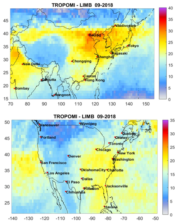
455 Figure 12. As Figure 11 (top left panel), but with zoom on China (top) and USA (bottom). Color indicates tropospheric ozone column in DU.
