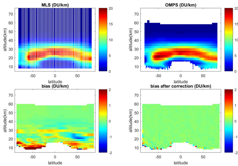
340 Figure 6. Illustration of the bias correction for September 2018. Upper panels: MLS and OMPS profiles averaged over latitude zones and over the month. Bottom panels: estimated biases before (left) and after (right) bias correction.
