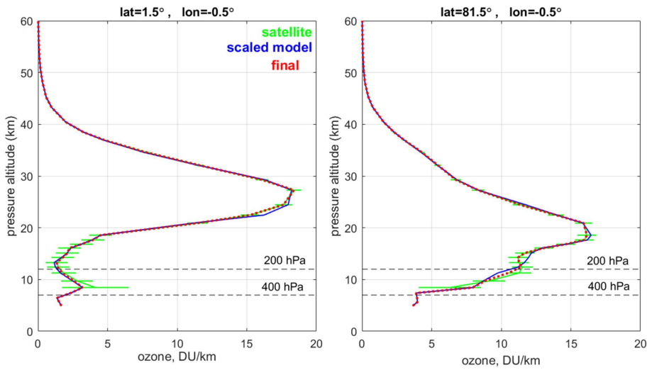
Figure 9. Illustration of transition to model-adjusted profiles at lower altitudes for tropical (left) and polar region (right). The vertical coordinate is pressure altitude z = 16 \log_{10}(P_0 / P) , where P_0=1013 hPa is the standard pressure and P is pressure in hPa.
