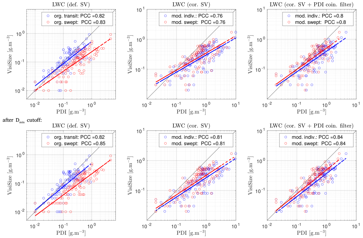
Figure 13. Comparison of the LWC results between the VisiSize and the PDI probe. From top-left to top-right, the plots show the raw data (based on the default sample volume for the VisiSize and the original DNC methods for the PDI), the data after modification, and the modified data after applying the coincidence filter to the PDI results. The scatter plots after applying the D_{\min} cutoff are shown in the second row. Each PDI method for the LWC computation is shown with a different color within the plots (each pair of blue/red circles: a selected measurement of \sim 15 min long). Dashed blue/red lines show the least squares regression (LSR), and the Pearson correlation coefficients (PCC) are displayed in the legend.
