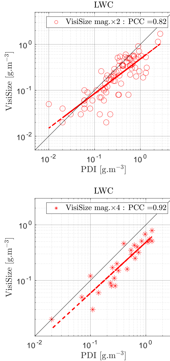
Figure 14. The LWC comparison between the two instruments, with cases using different lens magnification settings for the VisiSize ( \times 2 and \times 4 ), plotted separately. The results after applying all modifications and filters to the data and application of the PVC factor to the modified swept volume method of the PDI are shown here. Each circle/star represents a single measurement of \sim 15 min long. Dashed red lines show the least squares regression (LSR), and the Pearson correlation coefficient (PCC) is shown in the legend.
