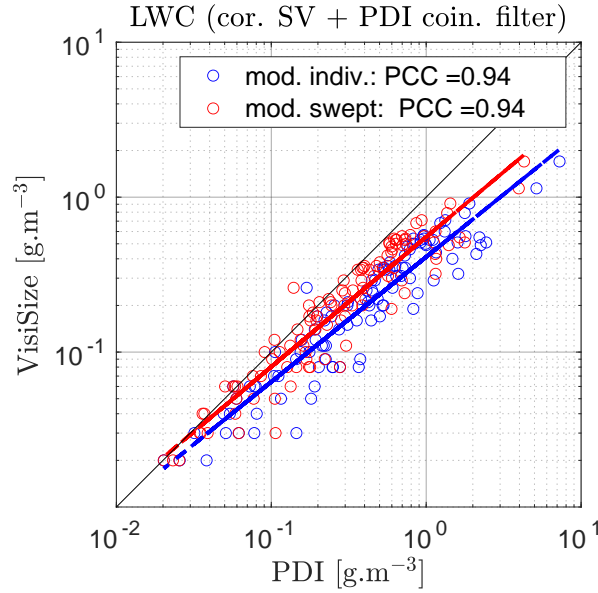
Figure 16. Comparison of the LWC results between the VisiSize and the PDI probe after adjusting the DNCs from the PDI using the reciprocal fit ( y = \frac{a}{x+b} ; see Figure 10). The data are shown after correction of the SV, applying the coincidence filter to the PDI results, and D_{\min} cutoff to both instruments' data. Each PDI method for the LWC computation is shown with a different color within the plot (each pair of blue/red circles: a selected measurement of \sim 15 min long). Dashed blue/red lines show the least squares regression (LSR), and the Pearson correlation coefficients (PCC) are displayed in the legend.
