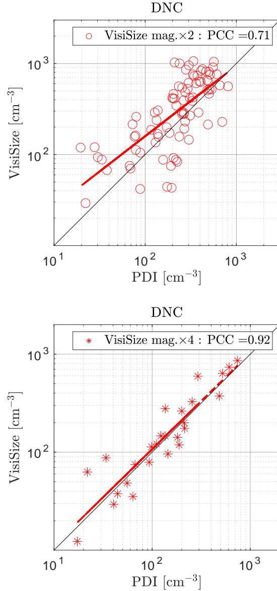
Figure 11. The DNC comparison between the two instruments, with cases using different lens magnification settings for the VisiSize ( \times 2 and \times 4 ), plotted separately. The results after applying all modifications and filters to the data and application of the PVC factor to the modified PDI swept volume method are shown here. Each circle/star represents a single measurement of \sim 15 min long. Dashed red lines show the least squares regression (LSR), and the Pearson correlation coefficient (PCC) is shown in the legend.
