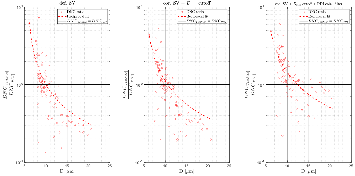
Figure 10. The DNC ratio of the VisiSize to the PVC-PDI as a function of the arithmetic mean diameter size. Panels from left to right show the raw data (using the default sample volume for the VisiSize), the results after the SV correction and the D_{\min} cutoff, and the results after additionally applying the coincidence filter to the PDI data. Each circle represents a single measurement of \sim 15 min long. The reciprocal fit curves ( y = \frac{a}{x+b} ) and the 1:1 ratio are shown with the dashed and black horizontal lines, respectively.
