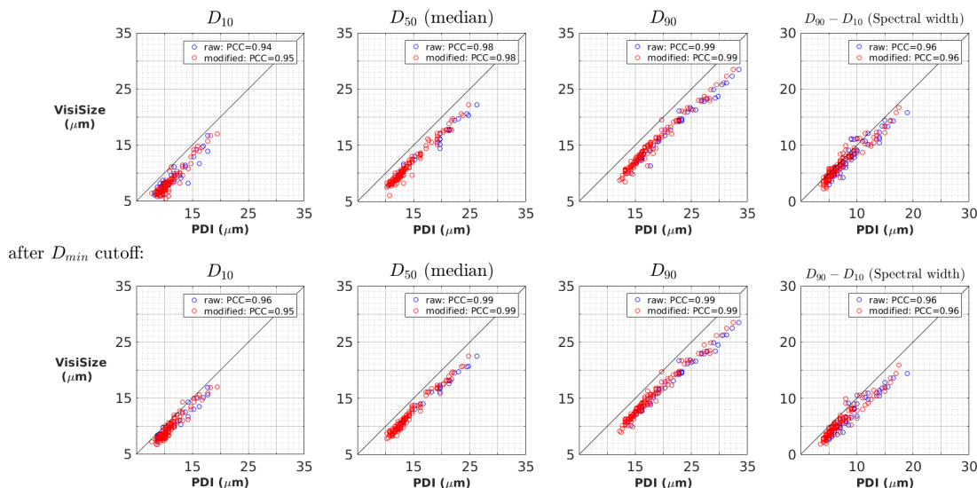
Figure 7. Comparison between the VisiSize and the PDI probe regarding the diameter size percentiles ( D_{10} , D_{50} , and D_{90} ) as well as the spectral width ( D_{90} - D_{10} ) of cloud droplets. Each pair of blue/red circles indicates the raw/modified data for a selected measurement of \sim 15 min long. The second row shows each plot after applying the D_{\min} cutoff to the data. Pearson correlation coefficients (PCC) are also shown in the legend.
