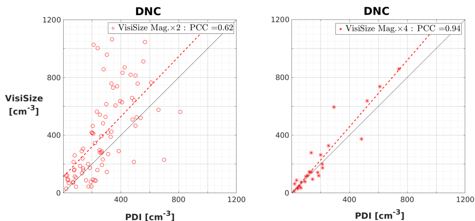
Figure 11. The DNC comparison between the two instruments, with cases using different lens magnification settings for the VisiSize ( \times 2 and \times 4 ), plotted separately. The results after applying all modifications and filters to the data and application of the PVC factor to the modified PDI swept volume method are shown here. Each circle/star represents a single measurement of \sim 15 min long. Dashed lines show the least squares regression (LSR), and the Pearson correlation coefficient (PCC) is shown in the legend.
