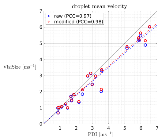
Figure 8. Comparison of the mean droplet velocity between the VisiSize and the PDI probe. Each pair of blue/red circles indicates the raw/modified data for a selected measurement of \sim 15 min long. Dashed lines show the least squares regression (LSR), and the Pearson correlation coefficients (PCC) are displayed in the legend.
