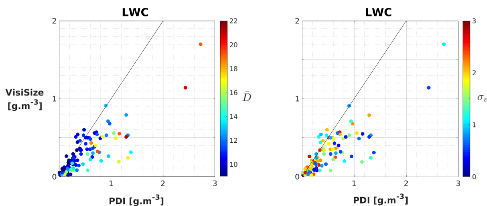
Figure 15. The LWC comparison between the two instruments, while the mean diameter spectra (left panel) and the standard deviation of velocity spectra (right panel) are also compared between the selected cases. The results after applying all modifications and filters to the data, and with application of the PVC factor on the modified swept volume method of the PDI are shown here. The mean diameters and the velocity standard deviations are taken from the VisiSize and the PDI data, respectively. Each circle represents a single measurement of \sim 15 min long.
