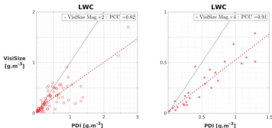
Figure 14. The LWC comparison between the two instruments, with cases using different lens magnification settings for the VisiSize ( \times 2 and \times 4 ), plotted separately. The results after applying all modifications and filters to the data and application of the PVC factor to the modified swept volume method of the PDI are shown here. Each circle/star represents a single measurement of \sim 15 min long. Dashed lines show the least squares regression (LSR), and the Pearson correlation coefficient (PCC) is shown in the legend.
