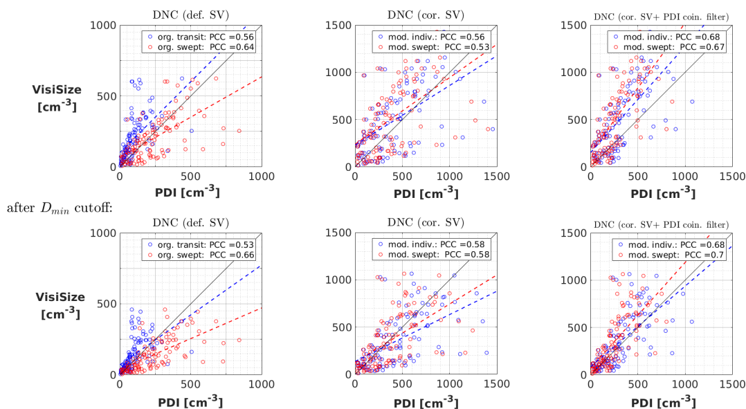
Figure 9. Comparison of the DNC results between the VisiSize and the PDI probe. From top-left to top-right, the plots show the raw data (based on the default sample volume for the VisiSize and the original DNC methods for the PDI), the data after modification, and the modified data after applying the coincidence filter to the PDI results. The scatter plots after applying the D_{min} cutoff are shown in the second row. Each PDI method for the DNC computation is shown with a different color within the plots (each pair of blue/red circles: a selected measurement of \sim 15 min long). Dashed lines show the least squares regression (LSR), and the Pearson correlation coefficients (PCC) are displayed in the legend.
