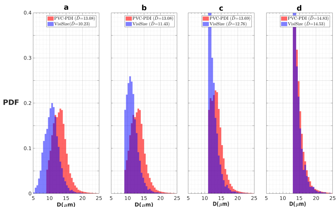
Figure 5. Probability distributions of cloud droplet size collected with the VisiSize and the PDI probe during a measurement on 13th July 2019 15:36 – 15:51. The distributions were truncated at progressively large values of droplet diameters for each plot: (a) D > 0 \mu\text{m} , (b) D > 9 \mu\text{m} , (c) D > 11 \mu\text{m} , and (d) D > 13 \mu\text{m} . The resulting arithmetic mean diameters for each instrument are shown in the legend.
