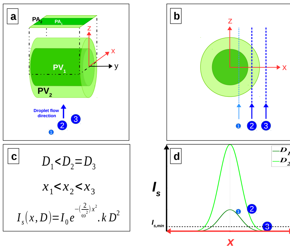
Figure 2. (a): Schematic representation of the cylindrical effective probe volume (PV) and probe area (PA) of the PDI for two different sizes of three passing droplets; (b): side view of panel (a) showing trajectories of the droplets located at different positions ( x ) from the yz plane; (c): relationship between size ( D ) and position ( x ) of the droplets along with the formula of the scattered intensity ( I_s ) as a function of x and D (where k is an instrument constant); (d): qualitative graphs of I_s - x illustrating the scattered intensity of each droplet based on its x and D as well as the minimum I_s below which a droplet cannot be detected.
