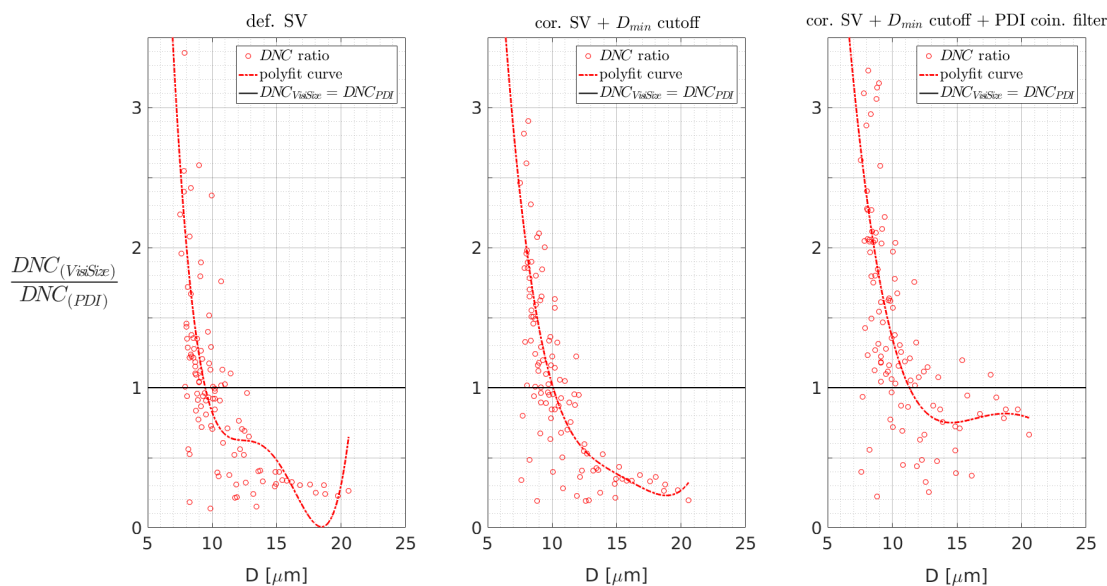
Figure 10. The DNC ratio of the VisiSize to the PVC-PDI as a function of the arithmetic mean diameter size. Panels from left to right show the raw data (using the default sample volume for the VisiSize), the results after the SV correction and the D_{\min} cutoff, and the results after additionally applying the coincidence filter to the PDI data. Each circle represents a single measurement of \sim 15 min long. The polynomial fit curves and the 1:1 ratio are shown with the dashed and black horizontal lines, respectively.
