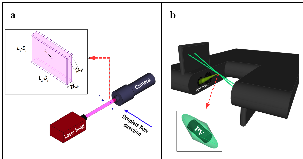
Figure 1. Schematic representation of (a): the VisiSize setup and a magnified sample volume (SV) around a droplet, comparing the default and corrected depth of fields ( z_{def} vs. z_{95} ); (b): a PDI probe with the magnified illustration of the cylindrical probe volume (PV) within the intersection of two laser beams where the light from the passing droplets is scattered into the receiver.
