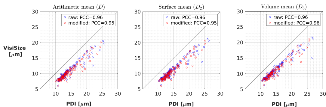
Figure 6. Comparison of cloud mean droplet diameter between the VisiSize and the PDI probe. Scatter plots of the arithmetic mean ( \bar{D} ), surface mean ( D_2 ) and volume mean ( D_3 ) are shown from left to right. Each pair of blue/red circles indicates the raw/modified data for a selected measurement of \sim 15 min long. Pearson correlation coefficients (PCC) are also shown in the legend as an index of the linear correlation.
