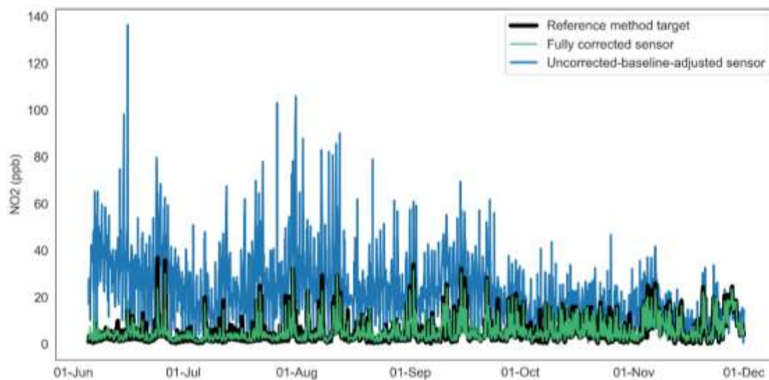
Figure 9. Time series of uncorrected-baseline-normalised-adjusted, fully corrected sensor observations and reference method observations for NO 2 St Ebbe's Oxford 2020.
