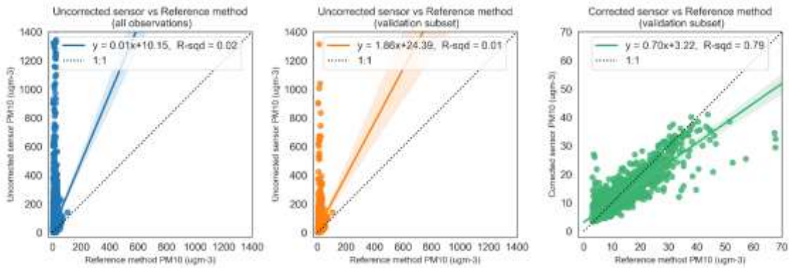
665 Figure 7. Relationship between uncorrected, RF model corrected sensor and reference method observations for PM 10 , the dotted line shows the unity slope.
