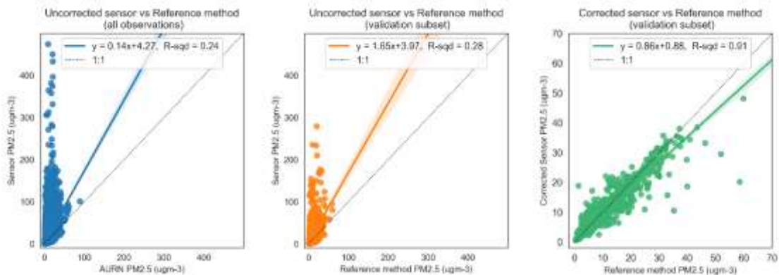
670 Figure 8. Relationship between uncorrected, RF model corrected sensor and reference method observations for PM 2.5 , the dotted line shows the unity slope.
