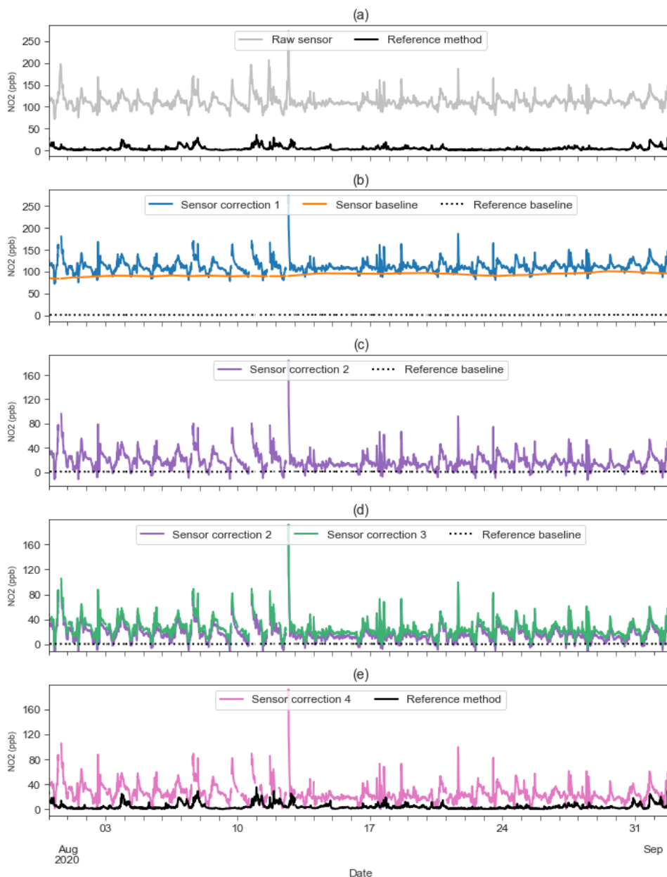
Figure 5. Illustrative impacts of each stage in the sensor baseline offset correction model upon 15-minute mean sensor observations, St Ebbe's, August 2020. (a) Raw sensor signal & reference method, (b) Correction 1- Application of empirical filters for anomaly & outlier removal, (c) Correction 2 - Baseline offset correction, (d) Correction 3 - Compensation for efficacy of baseline offset correction, (e) Correction 4 - Removal of residuals.
