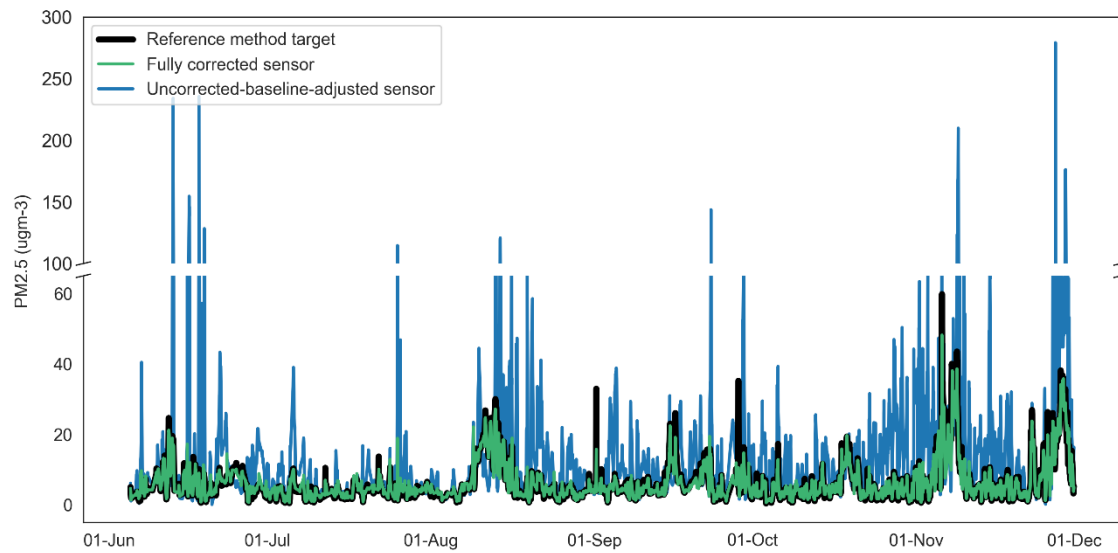
650 Figure 11. Time series of uncorrected-baseline-normalised, fully corrected sensor observations and reference method observations for PM 2.5 St Ebbe's Oxford 2020.
