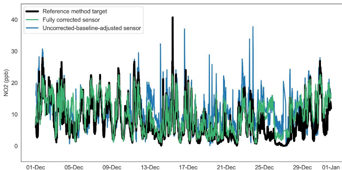
Figure 12. Time series of uncorrected-baseline-adjusted, fully corrected sensor observations and reference method observations for NO 2 St Ebbe's Oxford, unseen data, December 2020.
