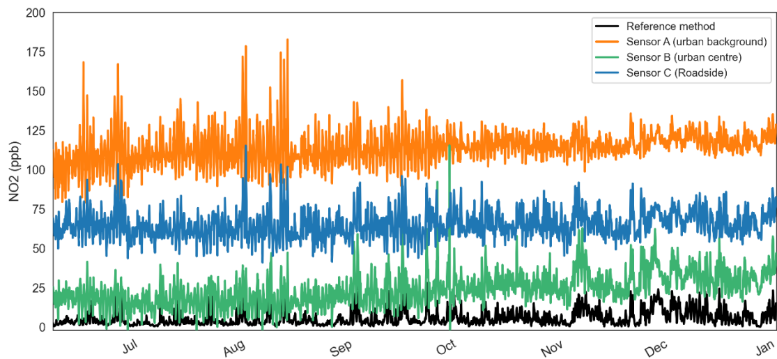
Figure 4. Three hour rolling mean raw low-cost sensor and reference method NO 2 time series at three locations in Oxford 2020.
