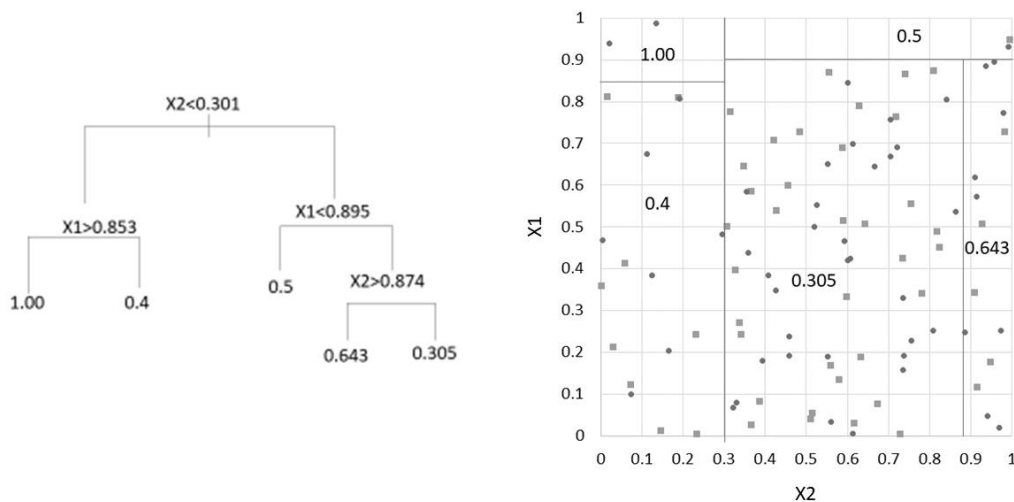
Figure 1: Visual representation of a generic, two variable Decision Tree regression problem (left) and its mapping on to a parameter space for the independent variables (right).
