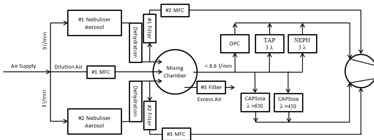
Figure 1. Experimental setup for the measurements. Flame soot measurements were done with a combustion flame source replacing #2 Nebuliser.
