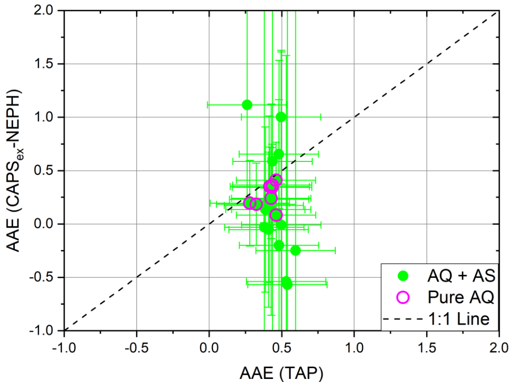
Figure 11. Scatter plot of AAE(CAPS, NEPH) measurements compared to AAE(TAP) measurements for pure AQ and AQ/AS external mixtures. Measured precision error bars are shown for individual AQ/AS externally mixed measurements.
