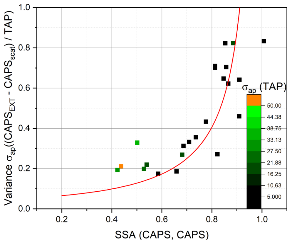
Figure 6. Variance of the measured absorption coefficients [ \sigma_{ap}(\text{CAPS, CAPS}) ] / \sigma_{ap}(\text{TAP}) ] for Differential Method calculations relative to TAP measurements for AQ and AS external mixtures. The ratios are plotted against the aerosol measured SSA values [SSA(CAPS, CAPS)]. The red line represents the calculated relative errors using Gaussian error propagation of the uncertainties of the DM Method with 1 as 100%..
