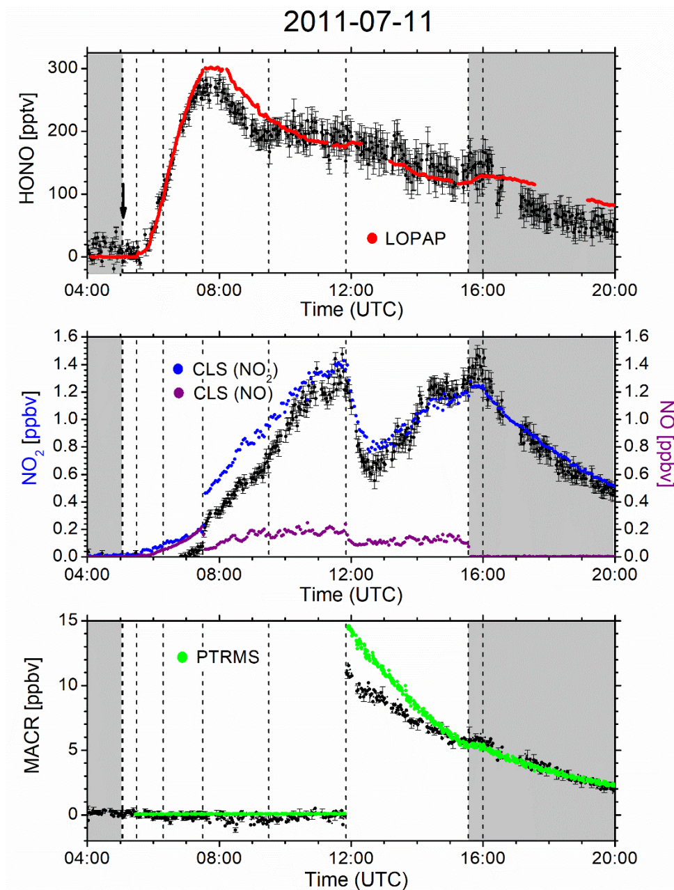
Figure 2(a): Time-dependent HONO, NO 2 and MACR mixing ratios measured by IBBCEAS (black trace) at SAPHIR on 11 July 2011. The NO mixing ratios (purple) measured by the CLS instrument are also shown. Dashed vertical lines indicate changes in the chamber conditions according to the experimental protocol: Overnight flushing of chamber with zero air stopped (5:03), roof opened (5:05), start of humidification (5:30), end of humidification (6:18), 40 ppbv O 3 (7:30), 750 ppbv CO (09:30), MACR (11:51), roof closing (15:33), flushing with zero air started (16:00). IBBCEAS data taken in the near-UV region of the spectrum (352-386 nm) are compared to LOPAP (red), CLS (blue) and PTRMS (green) data. The vertical black arrow indicates the time when I_0 was measured (generally for 10 min).
