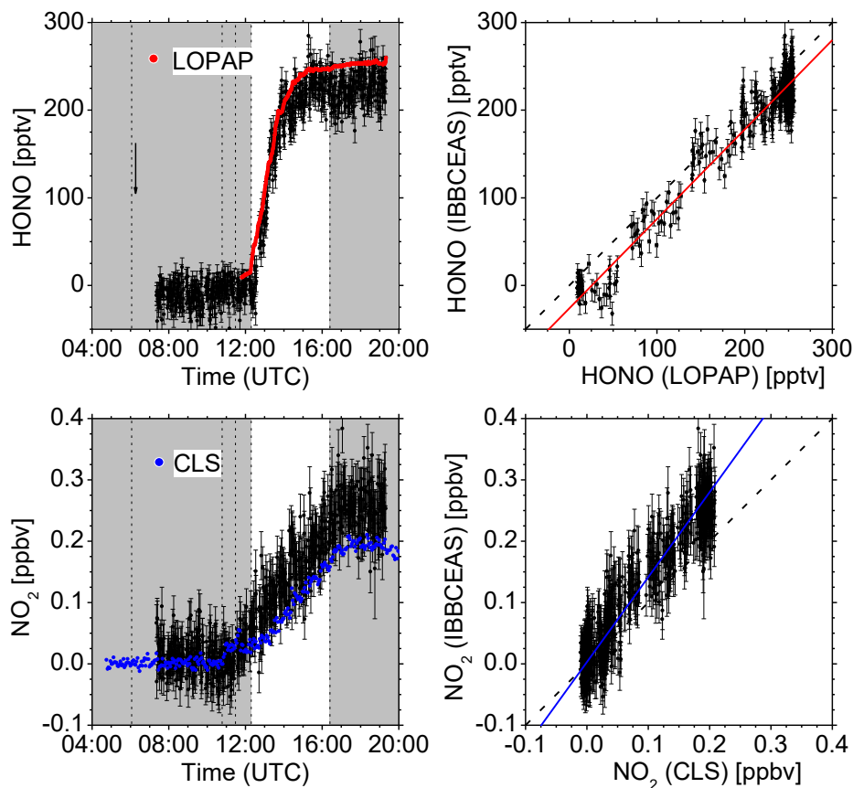
Figure 4: Left panels: Time-dependent HONO and NO 2 mixing ratios measured at SAPHIR on 6 October 2011. Dashed vertical lines indicate changes in the chamber conditions according to the experimental protocol: Overnight flushing stopped (6:04), start humidification (10:47), stop humidification (11:29), roof opening (12:18), roof closing (16:24). IBBCEAS data taken in the near-UV region of the spectrum (352-386 nm) are compared to LOPAP (red) and CLS (blue) data. The vertical black arrow indicates the time when I_0 was measured (generally for 10 min). Right panels: Correlation plots of two instruments being compared against IBBCEAS. The dashed line represents the identity, the colored solid lines are linear regressions to the data. Results are listed in Table 1.
