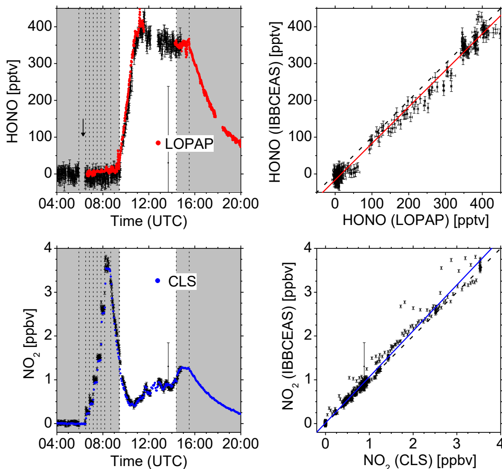
Figure 3: Left panels: Time-dependent HONO and NO 2 mixing ratios measured at SAPHIR on 5 October 2011. Dashed vertical lines indicate changes in the chamber conditions according to the experimental protocol: Overnight flushing stopped (5:55), 250 pptv NO 2 (6:30 and 6:50), 500 pptv NO 2 (7:10 and 7:30), 1 ppbv NO 2 (7:50 and 8:10), start humidification (8:41), stop humidification (9:25), roof opening (9:27), roof closing (14:23), flushing started (15:31). IBBCEAS data taken in the near-UV region of the spectrum (352–386 nm) are compared to LOPAP (red) and CLS (blue). The vertical black arrow indicates the time when I_0 was measured (generally for 10 min). Right panels: Correlation plots of two instruments being compared against IBBCEAS. The dashed line represents the identity, the colored solid lines are linear regressions to the data. Results are listed in Table 1.
