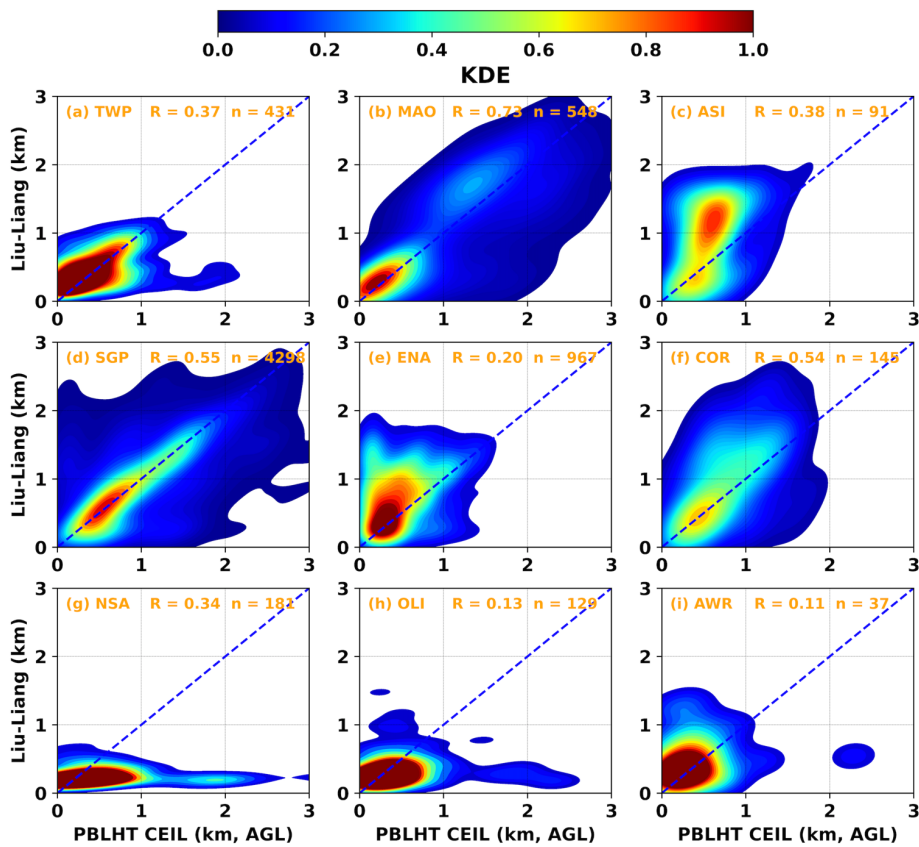
705 Figure 6: Kernel distribution estimate (KDE) for PBLHT CEIL and PBLHT Liu-Liang under LLC-free unstable boundary layer conditions at the nine ARM observatories. Blue dashed lines are the 1:1 line. R is the correlation coefficient and n is the sample number. The KDE is derived with a bin size of 0.1 km.
