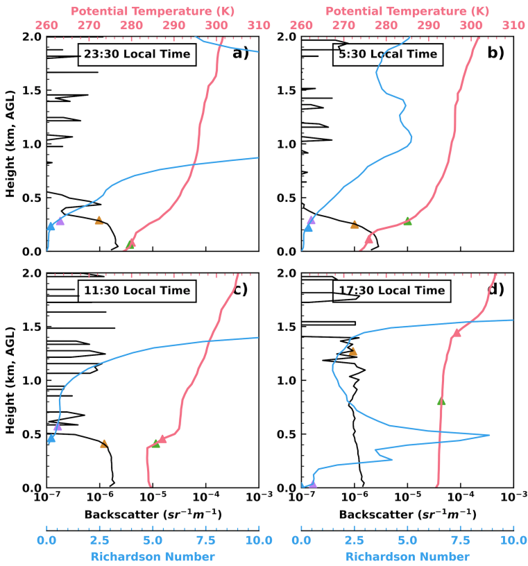
675 Figure 3: Ceilometer backscatter coefficient, radiosonde-derived potential temperature and Richardson number profiles at the radiosonde launching time of a) 23:30 Local Time (LT) on February 9; b) 5:30 LT on February 10; c) 11:30 LT on February 10; and d) 17:30 LT on
