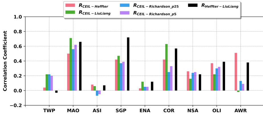
Figure 9: similar to Figure 5, but for LLC unstable boundary layer conditions.
