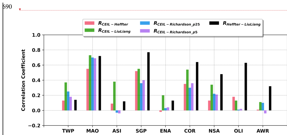
695 Figure 5: correlation coefficients between PBLHT CEIL and PBLHT Heffter ( R_{CEIL-Heffter} ), PBLHT Liu-Liang ( R_{CEIL-LiuLiang} ), PBLHT Richardson ( R_{CEIL-Richardson_{p25}} and R_{CEIL-Richardson_{p5}} ). Correlation coefficients between PBLHT Heffter and PBLHT Liu-Liang are also plotted ( R_{Heffter-LiuLiang} ).
