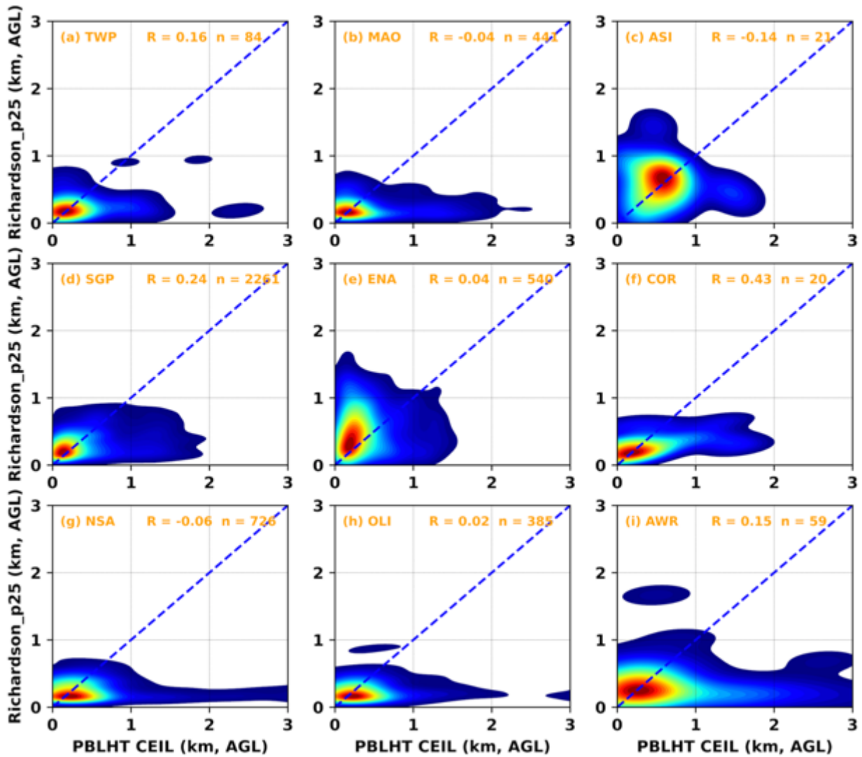
535 Figure 8: similar to Figure 6, but for PBLHT CEIL and PBLHT Richardson_p25 under LLC-free stable boundary layer conditions.
