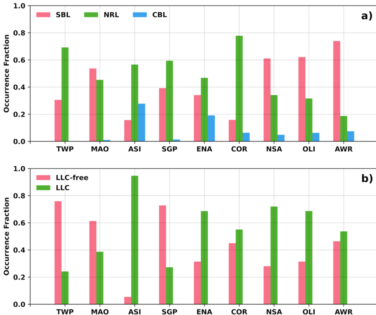
515 Figure 4: Occurrence fractions of a) different boundary layer regimes; b) low-level cloudy and cloud-free conditions at the nine ARM observatories during the time periods examined in this study. SBL, NRL, and CBL stand for stable boundary layer, neutral residual layer, and convective boundary layer correspondently in plot a). LLC-free and LLC stand for low-level cloud free and low-level cloudy conditions correspondently in plot b).
