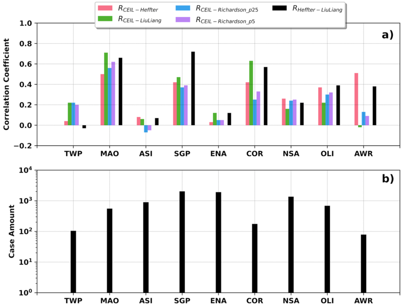
540 Figure 9: similar to Figure 5, but for LLC unstable boundary layer conditions.
