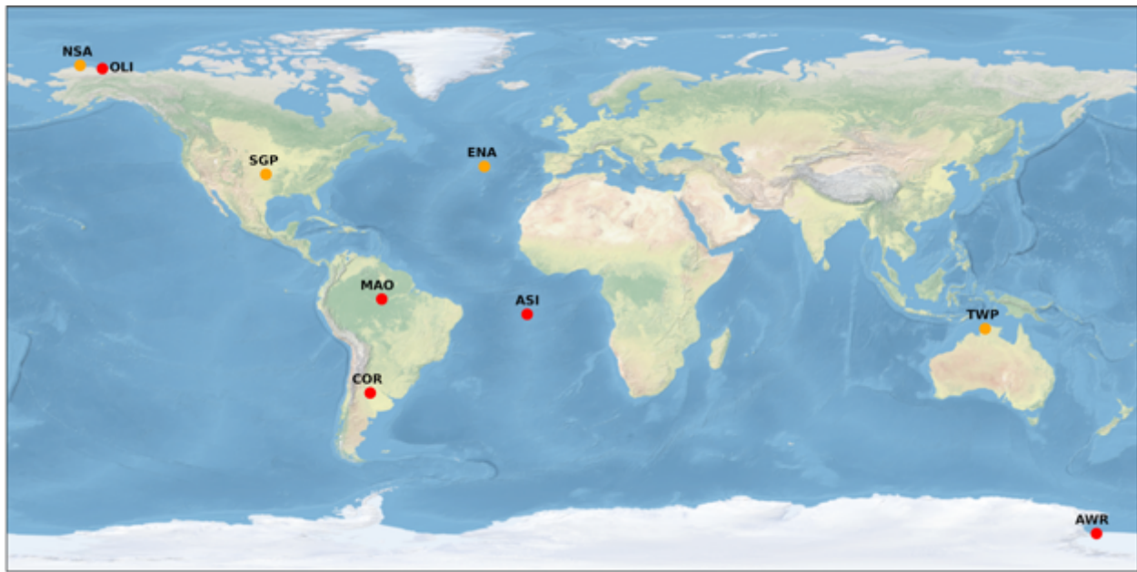
510 Figure 1: The geographical locations of ARM fixed-location observatories (orange circles) and AMF field campaign deployments (red circles).
