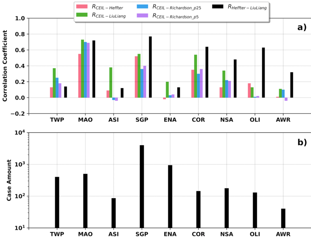
535 Figure 5: a) correlation coefficients between PBLHT CEIL and PBLHT Heffter ( R_{CEIL-Heffter} ), PBLHT Liu-Liang ( R_{CEIL-LiuLiang} ), PBLHT Richardson ( R_{CEIL-Richardson\_p25} and R_{CEIL-Richardson\_p5} ). Correlation coefficients between PBLHT Heffter and PBLHT Liu-Liang are also plotted ( R_{Heffter-LiuLiang} ); b) correspondent radiosonde amounts at ARM observatories under the LLC-free unstable boundary layer conditions.
