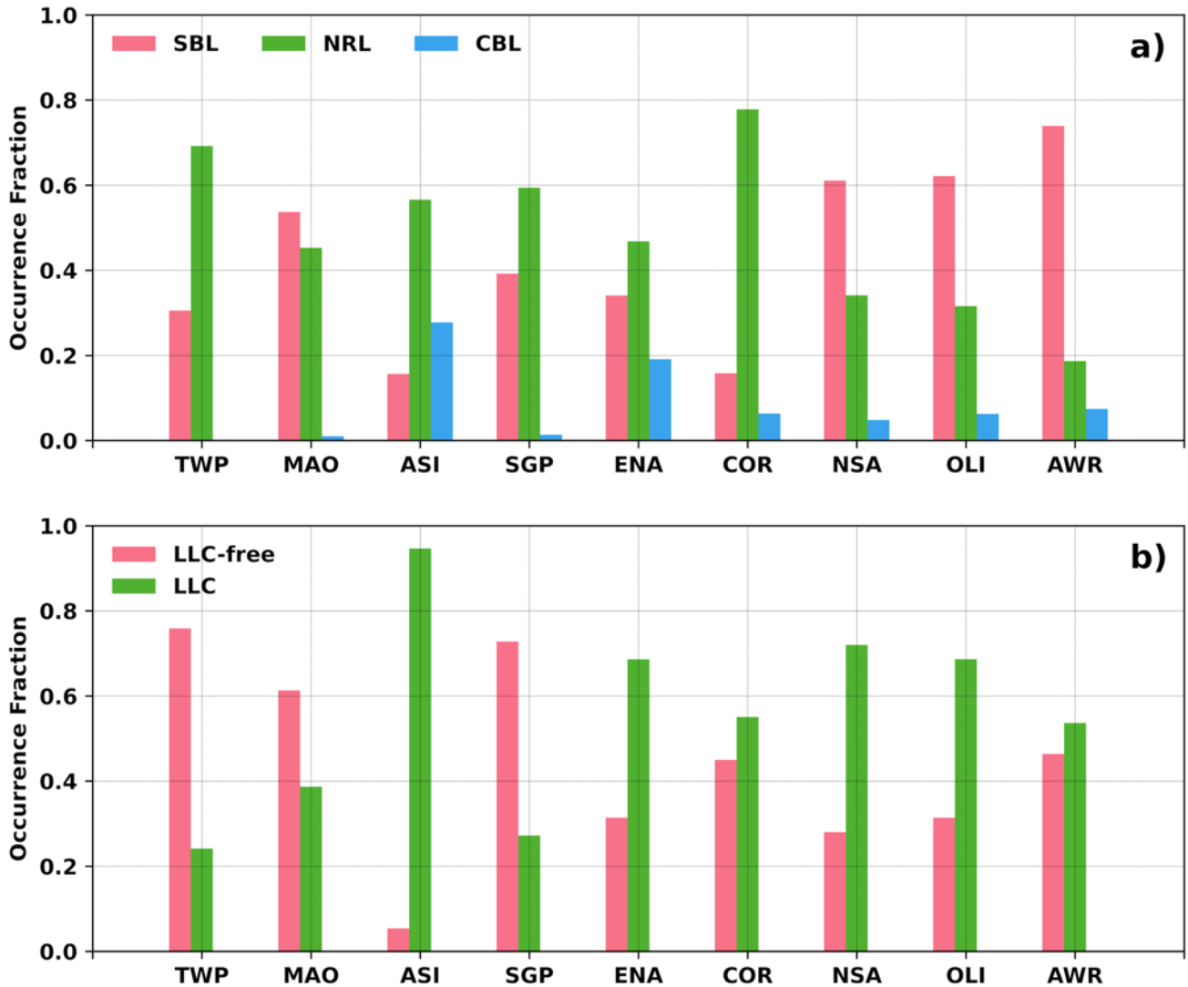
530 Figure 4: Occurrence fractions of a) different boundary layer regimes; b) low-level cloudy and cloud-free conditions at the nine ARM observatories during the time periods examined in this study. SBL, NRL, and CBL stand for stable boundary layer, neutral residual layer, and convective boundary layer correspondently in plot a). LLC-free and LLC stand for low-level cloud free and low-level cloudy conditions correspondently in plot b).
