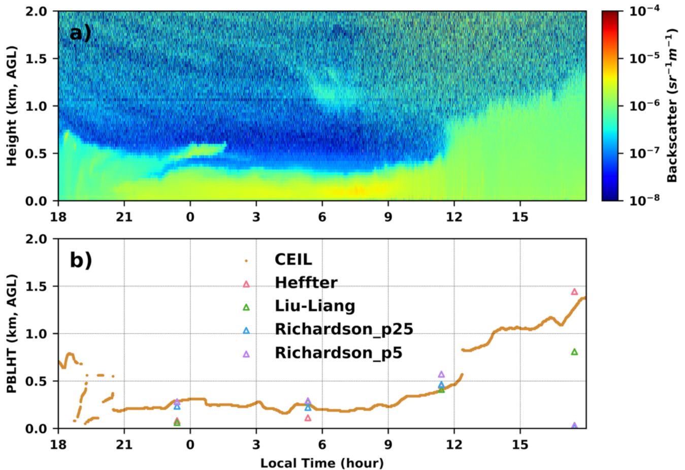
515 Figure 2: An example of estimated PBLHTs from ceilometer and the PBLHT-SONDE VAP on February 9-10, 2015, at the ARM SGP site. a) time-height cross section of ceilometer total attenuated backscatter coefficient; b) estimated PBLHTs from ceilometer measurements (labeled as ‘CEIL’) and the PBLHT-SONDE VAP including the Heffter (labeled as ‘Heffter’), Liu and Liang (labeled as ‘Liu-Liang’), and bulk Richardson number (using Ri_c of 0.25 is labeled as ‘Richardson_p25’ and using Ri_c of 0.5 is labeled as ‘Richardson_p5’) methods.
