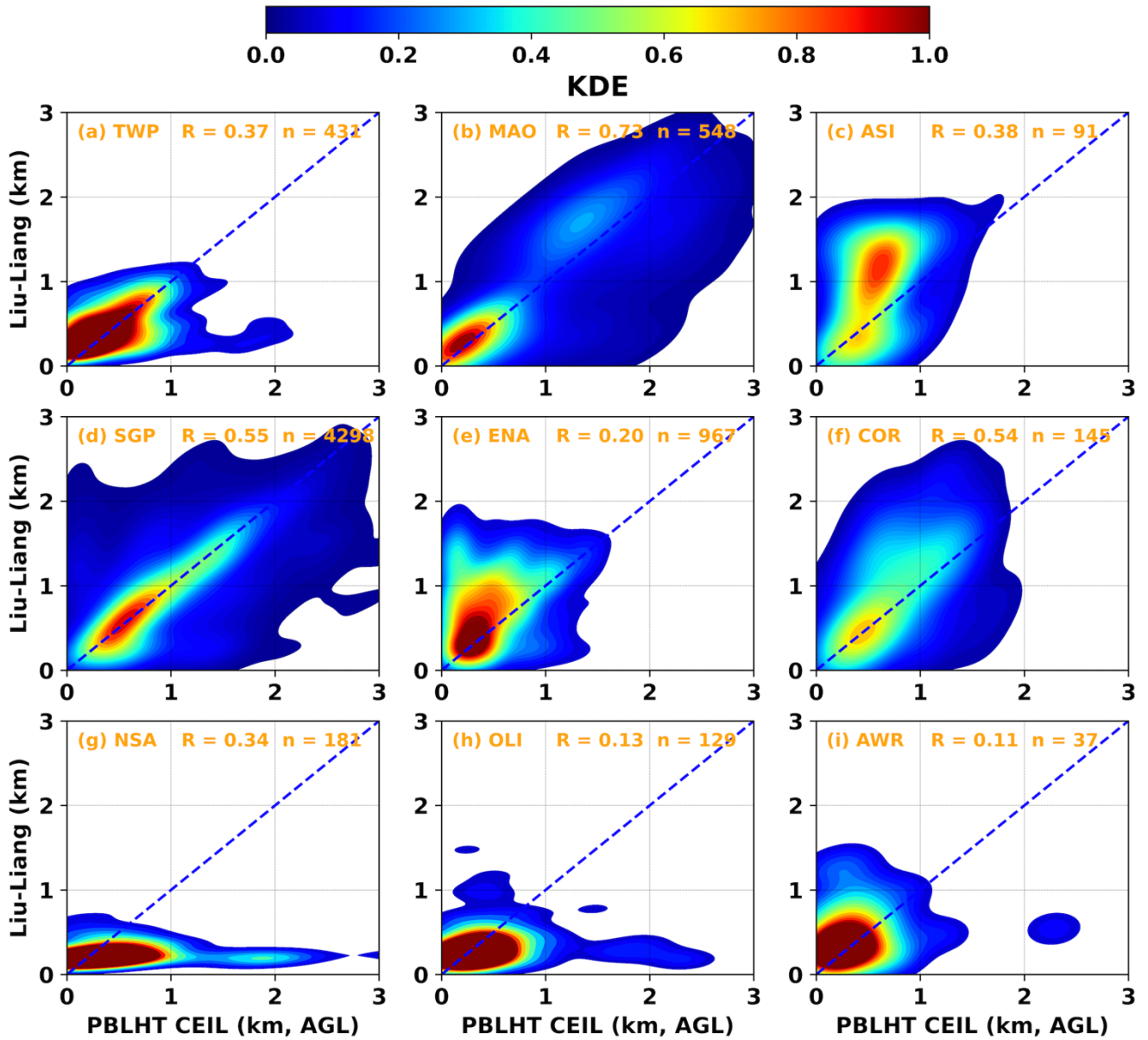
Figure 6: Kernel distribution estimate (KDE) for PBLHT CEIL and PBLHT Liou-Liang under LLC-free unstable boundary layer conditions at the nine ARM observatories. Blue dashed lines are the 1:1 line. R is the correlation coefficient and n is the sample number. The KDE is derived with a bin size of 0.1 km.
