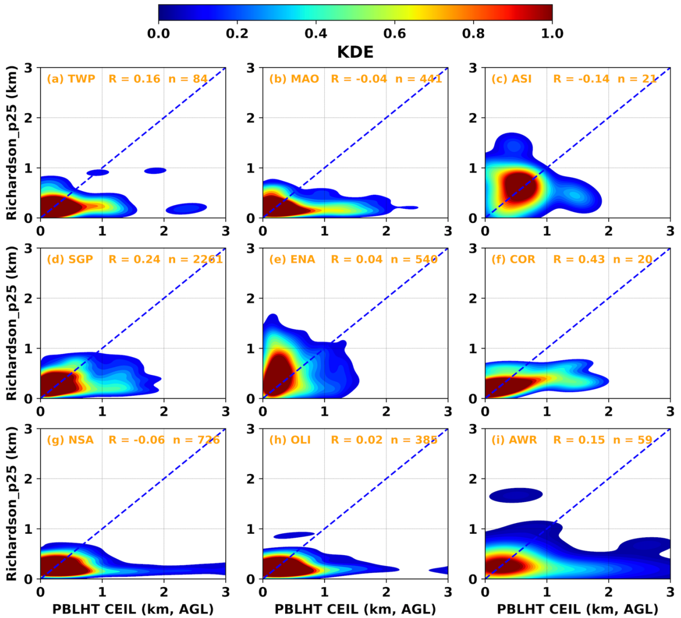
Figure 8: similar to Figure 6, but for PBLHT CEIL and PBLHT Richardson_p25 under LLC-free stable boundary
