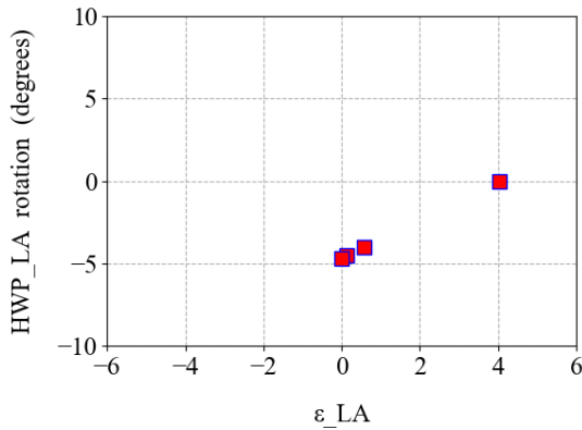
Figure C1. The test performed for zeroing \varepsilon_{LA} , for defining the polarization of i_{LA} with respect to the horizon.
