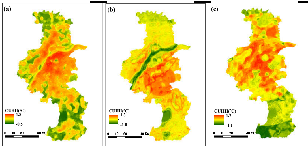
Figure 8: Spatial distribution of the CUHI in Nanjing: (a) 11 August 2013; (b) 2 September 2015; (c) 21 July 2017.
