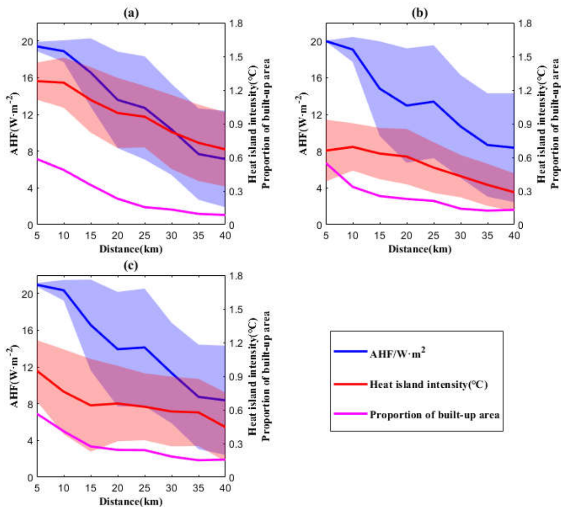
Figure 12: Changes in air temperature, anthropogenic heat flux (AHF) and the proportion of built-up areas with distance from the city center on (a) 11 August 2013, (b) 2 September 2015, and (c) 21 July 2017. Thick lines represent mean values, while shaded regions are the uncertainties of one standard value from the mean.
