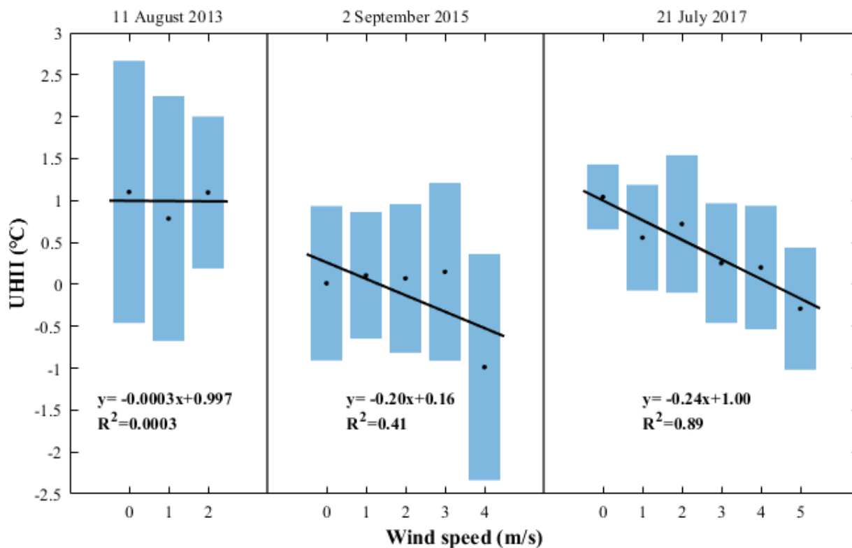
Figure 10: Relationship between urban heat island intensity (UHII) and wind speed around all meteorological stations on (a) 11 August 2013, (b) 2 September 2015, and (c) 21 July 2017. The black dots represent the mean UHII, while the bottom and top edges of the box indicate the uncertainties of one standard value from the mean
