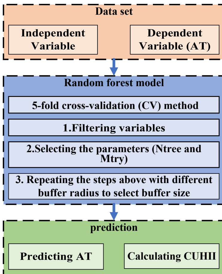
Figure 3: Flowchart for constructing the RF model and evaluating the CUHII (Canopy urban layer heat island intensity). Abbreviations: DEM, digital elevation model; AHF, anthropogenic heat flux; LULC, land use/land cover; IS, impervious surface; AT, air temperature; RF, Random Forest.
