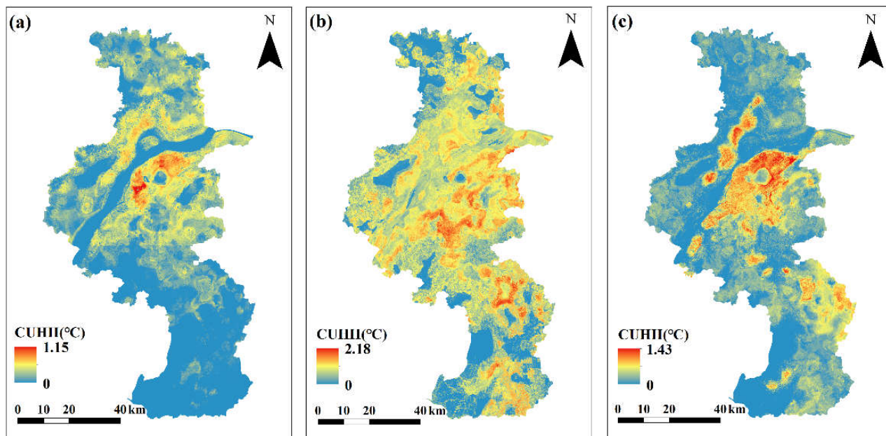
Figure 13: Spatial distribution of canopy urban heat island intensity (CUHII) in Nanjing during a heat wave period: (a) 12 August 2013; (b) 13 August 2013; (c) 14 August 2013.
