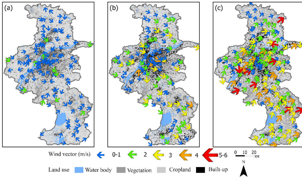
Figure 9: Wind vector field in Nanjing on (a) 11 August 2013, (b) 2 September 2015, and (c) 21 July 2017.
