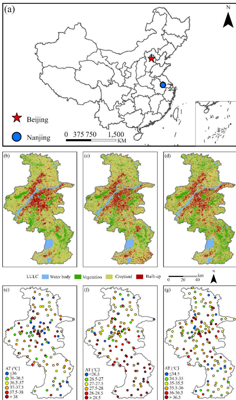
Figure 1: Land use/land cover of Nanjing city and locations of automatic meteorological stations in Nanjing with recorded air temperature: (a) location map of Nanjing in China; (b, e) 11:00 local time (LT) 11 August 2013; (c, f) 11:00 LT 2 September 2015; (d, g) 11:00 LT 21 July 2017.
