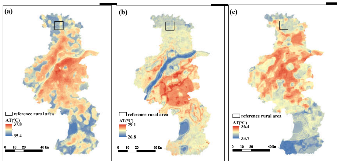
Figure 7: Spatial distribution of air temperature (AT) in Nanjing and the reference rural area: (a) 11 August 2013; (b) 2 September 2015; (c) 21 July 2017.
