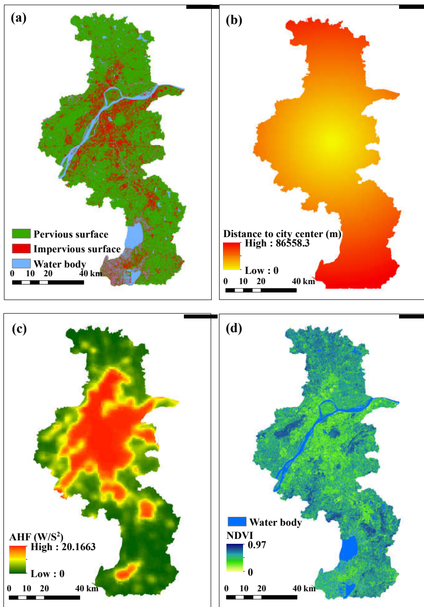
Figure 2: Spatial distribution of some environmental variables on 21 July 2017 in Nanjing city: (a) impervious surface; (b) distance from city center; (c) AHF (anthropogenic heat flux); (d) NDVI (normalized difference vegetation index).
