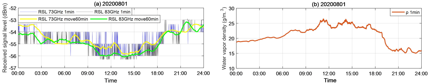
140 Figure 2: (a) Comparison of the link received signal level RSL before and after sliding on August 1, 2020, CST; (b) Water vapor density \rho calculated from weather station data.
