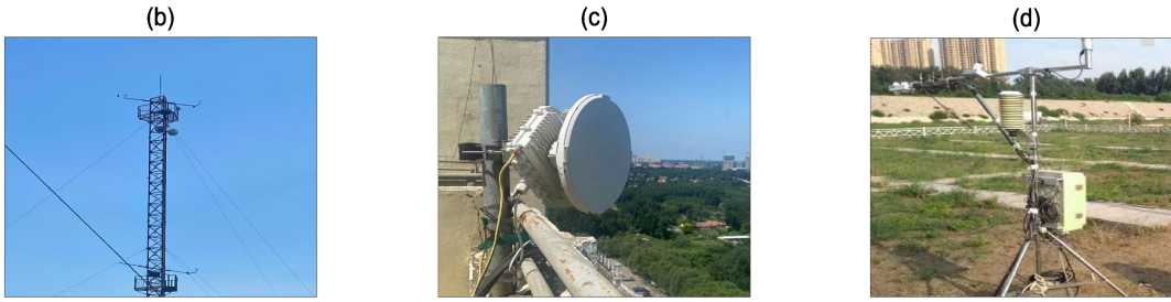
95 Figure 1: (a) Location of the E-band millimeter-wave link (from Baidu Maps); (b) The transmitter of the link; (c) The receiver of the link; (d) The automatic weather stations in the experiment.
