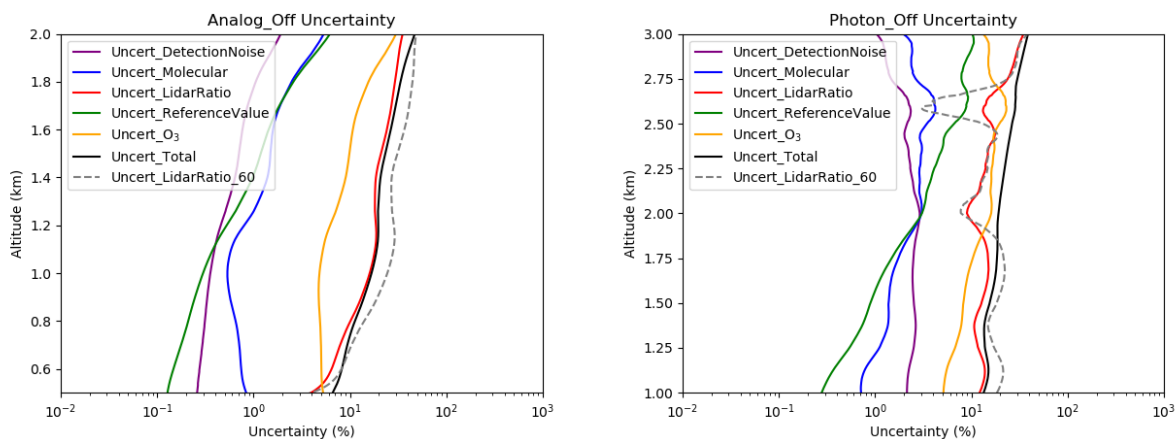
370 Figure 8: The uncertainty budget for the LMOL Analog channel (left) and the Photon channel (right) for August 28, 2018 afternoon retrieval. The uncertainties are attributed to different factors: detection noise (purple), molecular number density (blue), S_1 (red), reference value (green), uncertainty of O 3 (orange), total uncertainty (black). The uncertainty caused by using 60 sr as S_1 was shown in dashed gray line.
