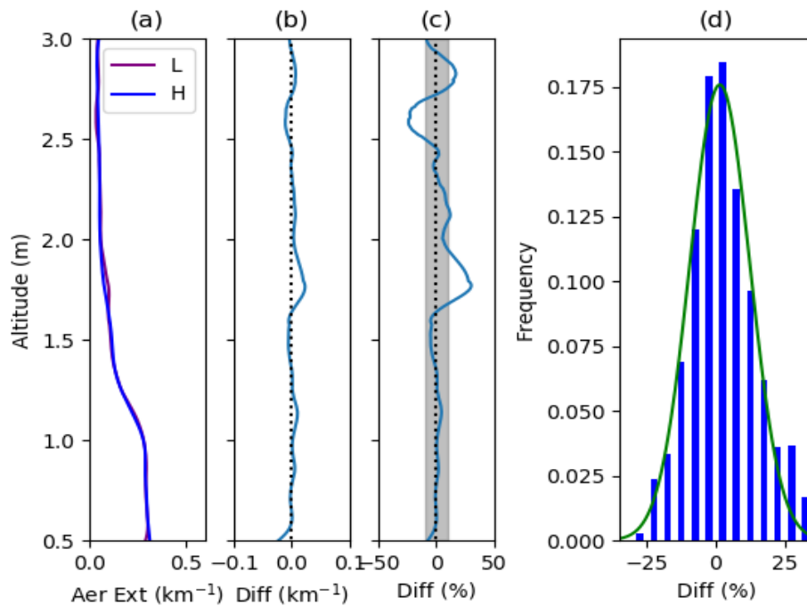
285 Figure 6: Comparison of the LMOL and HALO derived 292 nm aerosol extinction coefficient on August 28, 2018, afternoon at 13:17 EDT using the S_1 and AE selected in section 3.2. The HALO aerosol extinction profile is converted from 532 nm aerosol extinction product. (a) LMOL and HALO aerosol extinction; (b) difference between LMOL and HALO aerosol extinction; (c) The percent difference between LMOL and HALO aerosol extinction; and (d) The error (percentage difference) probability distribution function for all available comparison between 0.5-2.5 km for August 2018. The width between each bar shows 5% difference.
