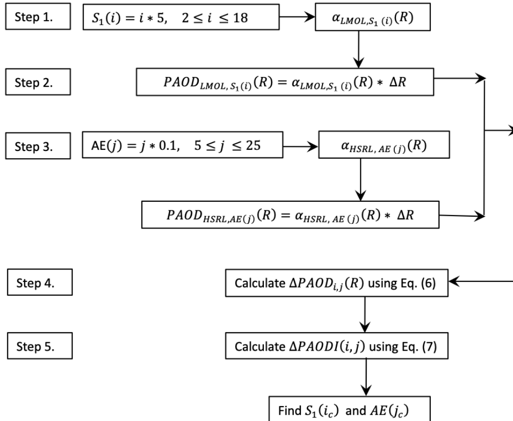
235 Figure 3: The flow chart for process of calculating the 292 nm S_1 and AE between 532 nm and 292 nm. “i” is the integer increment from 2 to 18 that used to calculate the S_1 to make the S_1 varies from 10 to 90. “j” is the integer increment from 5 to 25 that used to calculate the AE to make the AE varies from 0.5 to 2.5. “i” and “j” also could be the index of the calculated partial AOD.
