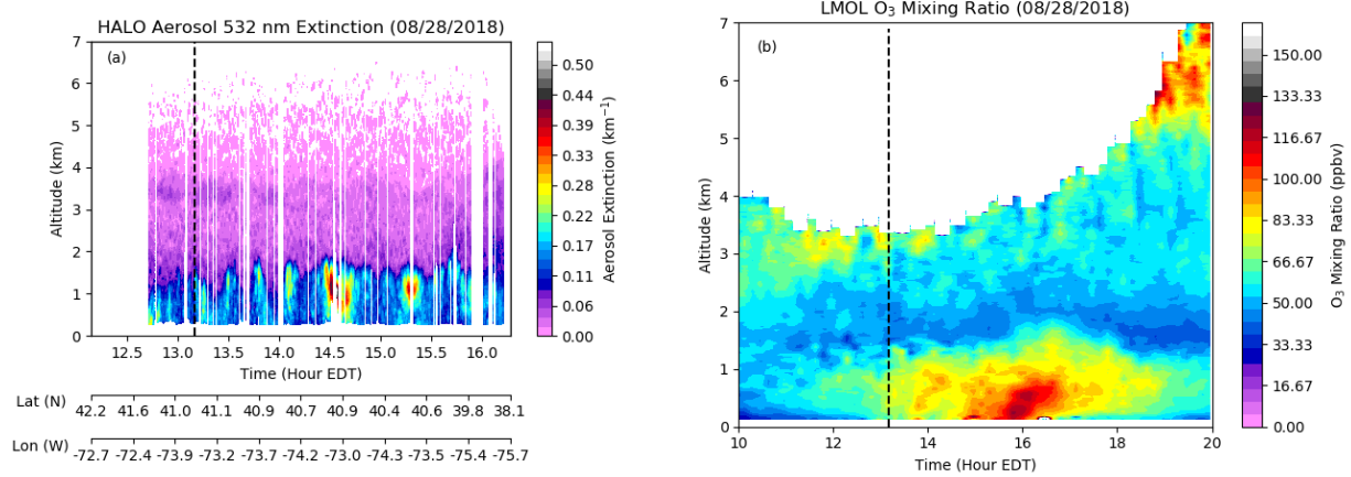
Figure S1: (a) The HALO aerosol extinction curtain plot on August 28 afternoon and (b) the LMOL O 3 measurement on August 28. The black vertical line shows the coincidence measurement when HALO overpass LMOL at 13.17 EDT.
