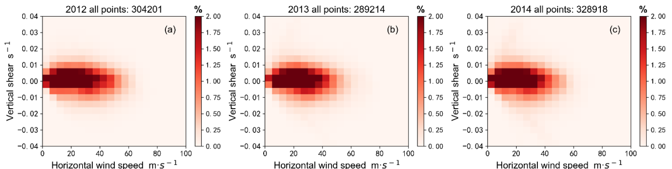
255 Figure 1. Two-dimensional frequency distribution characteristics of horizontal wind speed and vertical shear of horizontal wind speed within the height range of 3–19.8km above the Beijing MST radar station from 2012 to 2014.
