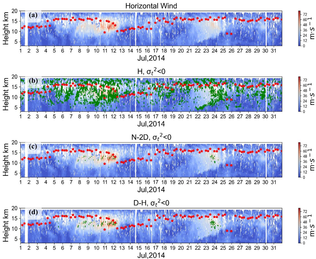
430 Figure 6. N-TKE distribution of three models over the Beijing MST radar site in July 2014: (a) horizontal wind speed; (b–d) area of N-TKE (green shading) for the (b) H model, (c) N-2D model and (d) D-H model. The red scattered points are the tropopause.
