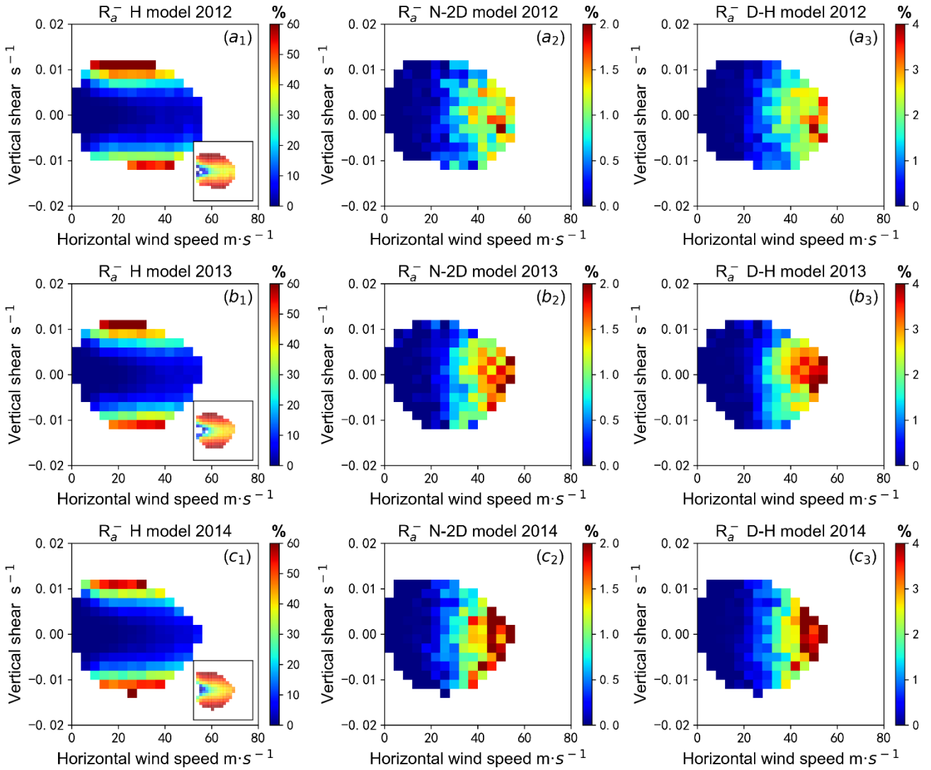
300 Figure 3. Distribution of R_a^- for the (a 1 ) H model, (a 2 ) N-2D model, and (a 3 ) D-H model in 2012. Panels (b 1 )–(b 3 ) and (c 1 )–(c 3 ) are the same as (a 1 )–(a 3 ) but for the results of the three models in 2013 and 2014, respectively. The subgraph at the lower right corner of (a 1 , b 1 , c 1 ) is the same as (a 1 , b 1 , c 1 ), but for \log_{10}(R_a^-) .
