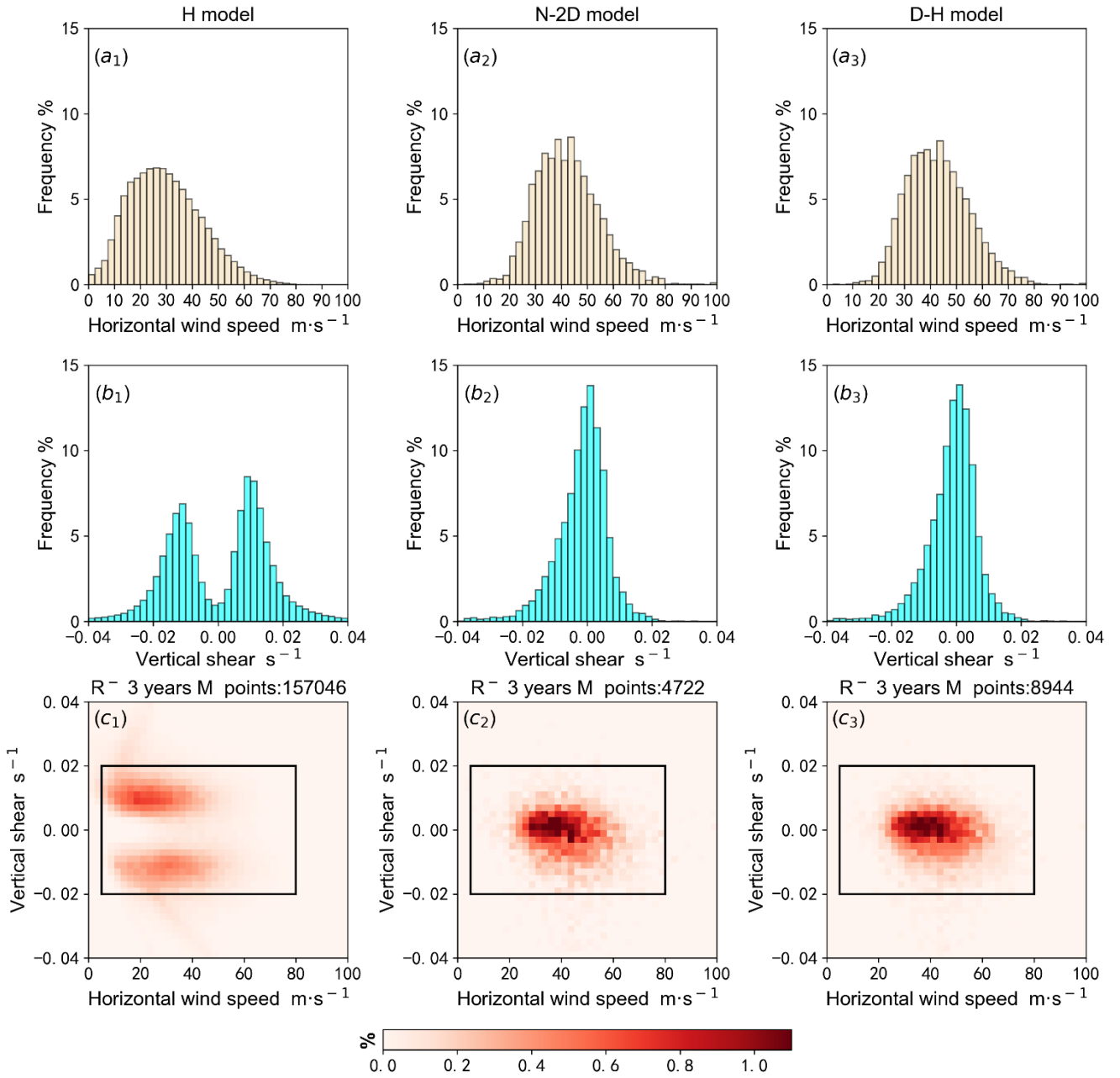
270 Figure 2. Frequency distribution of (a 1 –a 3 ) horizontal wind speed and (b 1 –b 3 ) the vertical shear of horizontal wind speed, along with (c 1 –c 3 ) the two-dimensional frequency distribution characteristics of horizontal wind speed and the vertical shear of horizontal wind speed for H model (a 1 , b 1 , c 1 ), N-2D model (a 2 , b 2 , c 2 ) and D-H model (a 3 , b 3 , c 3 ) when the turbulent kinetic energy is negative.
