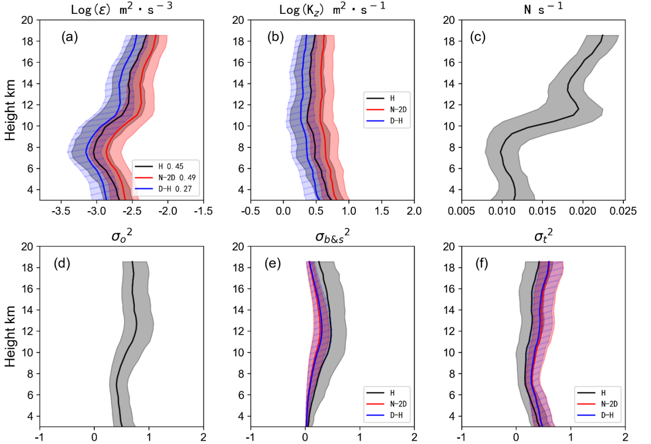
Figure 5. Profiles of (a) \epsilon , (b) K_z , (c) B-V frequency, (d) observation spectrum width, (e) beam and shear broadening, and (f) spectrum width caused by turbulence. The solid line is the median and the shaded area is the upper and lower quartiles. In panels (a, b, e, f), the black/red/blue solid lines and shaded areas represent the median and upper and lower quartiles of the H model/N-2D model/D-H model, respectively.
