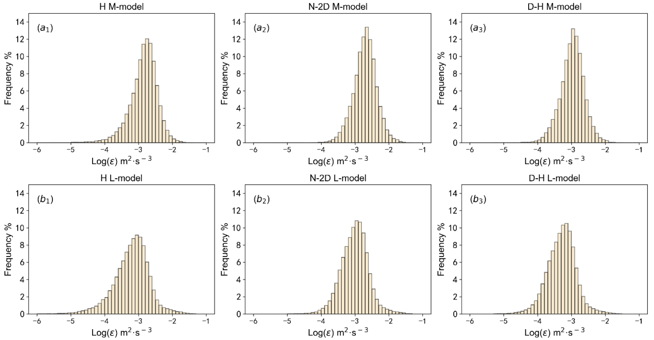
Figure 7. Distribution of \varepsilon in the middle and low mode of the Beijing MST radar in the range of 3–7.8 km from 2012–2014: ( a_1 – a_3 ) distributional characteristics of \varepsilon in the H model, N-2D model and D-H model (mid mode); ( b_1 – b_3 ) as in ( a_1 – a_3 ) but for low-mode data.
