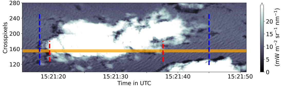
Figure 7. Cloud partly reaching into the FOV of the radar (orange swath), measured by the imager 1600 nm channel. Dashed lines indicate the along-track cloud length within the radar (red) and maximum along-track cloud length for the entire across-track extension (blue).
