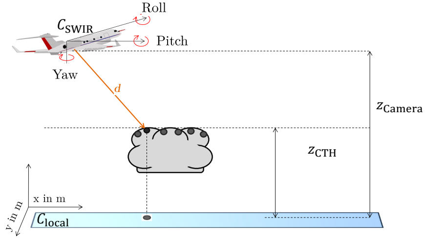
Figure 3. Illustration of the transformation from cloud pixels in the camera coordinate system C_{\text{SWIR}} into the local distance based reference system. Aircraft yaw, pitch and roll axes are defined in the top left-hand corner.
