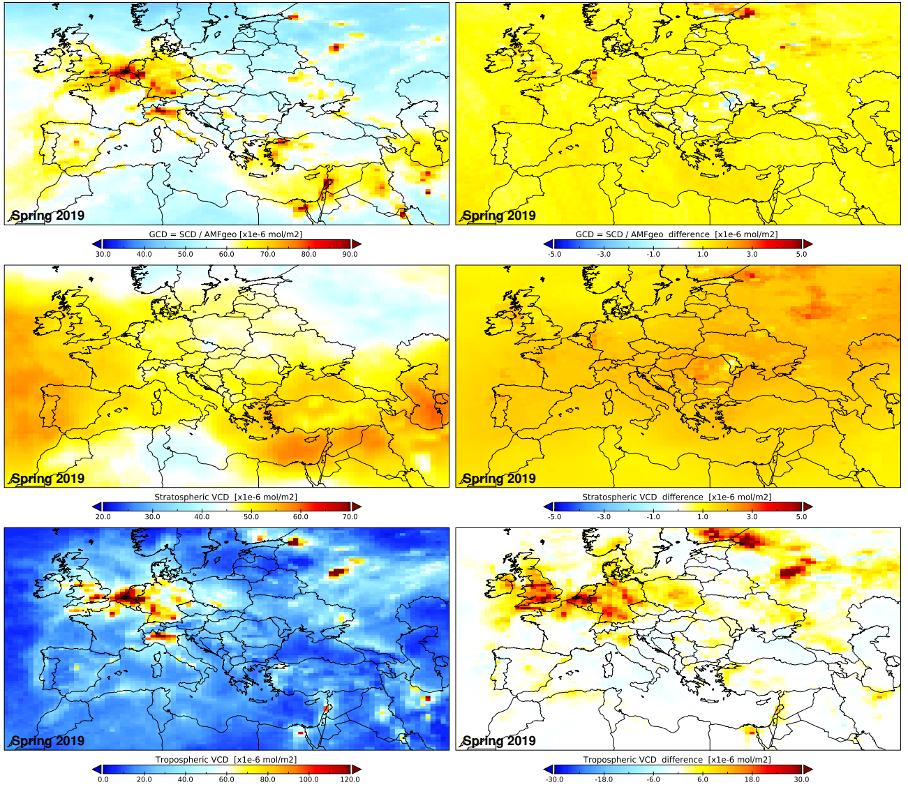
Figure 5. Maps of gridded data averaged over the Spring 2019 VCD period (cf. Table 1) of all ground pixels with valid retrieval: the \text{NO}_2 GCD (top row), stratospheric VCD (middle row) and tropospheric VCD (bottom row) values of the v2.1 data (left column) and the "DDS minus OFFL" difference (right column), all in \mu\text{mol m}^{-2} . The depicted area is longitude = [-15^\circ : +55^\circ] , latitude = [+27.5^\circ : +62.5^\circ] .
