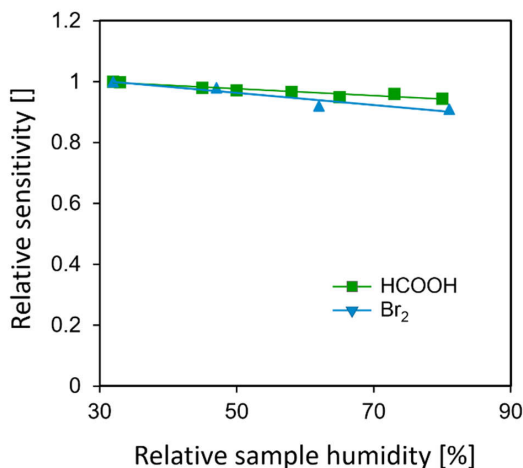
245 Figure 4: Relative sensitivities of formic acid (HCOOH) and bromine (Br 2 ) as a function of sample relative humidity (RH; T ambient = 22°C, added H 2 O flow: 18 sccm). Sensitivities are normalized to the driest conditions (RH=30%).
