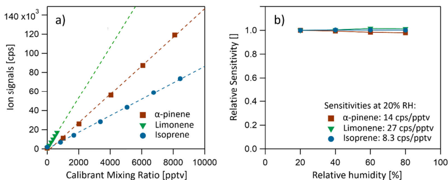
300 305 310 Figure 6: Calibrations in benzene mode; panel a) instrument response to selected biogenic calibrants (isoprene, C_5H_8 ; \alpha -pinene, C_{10}H_{16} ; limonene, C_{10}H_{16} ); panel b) sample humidity dependency of the calibrants
