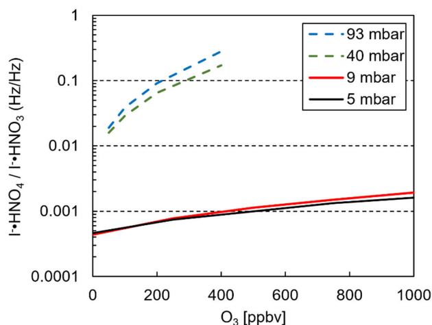
Figure 5: Ratio of \text{I} \cdot \text{HNO}_4 and \text{I} \cdot \text{HNO}_3 as a function of ozone mixing ratio of the sample gas. Solid lines: Instrument described in this work operating at pressures indicated in the legend; Dashed lines: Data from a standard I-CIMS operated at pressures indicated in the legend (40 and 93 mbar).
