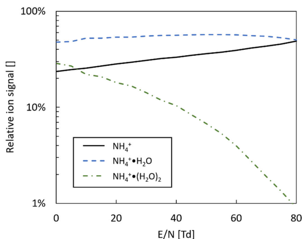
325 Figure 7: Reagent ion cluster distribution in ammonia mode as a function of reduced electric field (E/N). Drift tube pressure: 2 mbar; drift tube temperature: 60 °C.
