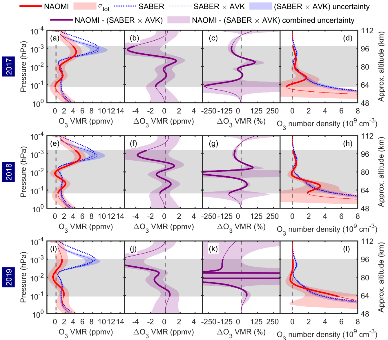
345 Figure 8: Mean ozone vertical profiles from NAOMI and SABER 9.6 \mu\text{m} observations during autumn twilight (within 15 September–15 November, 75^\circ \leq \text{SZA} at altitude 90 km \leq 110°) conditions in 2017 (a–d), 2018 (e–h), and 2019 (i–l). The second and third columns give the absolute and relative (%) differences (NAOMI minus SABER 9.6 \mu\text{m} ). The red, blue, and purple shading are the estimated uncertainties of the plotted parameters. The grey shaded regions and thicker sections of the plotted curves indicate the pressure and altitude ranges where \text{MR} \geq 0.8 .
