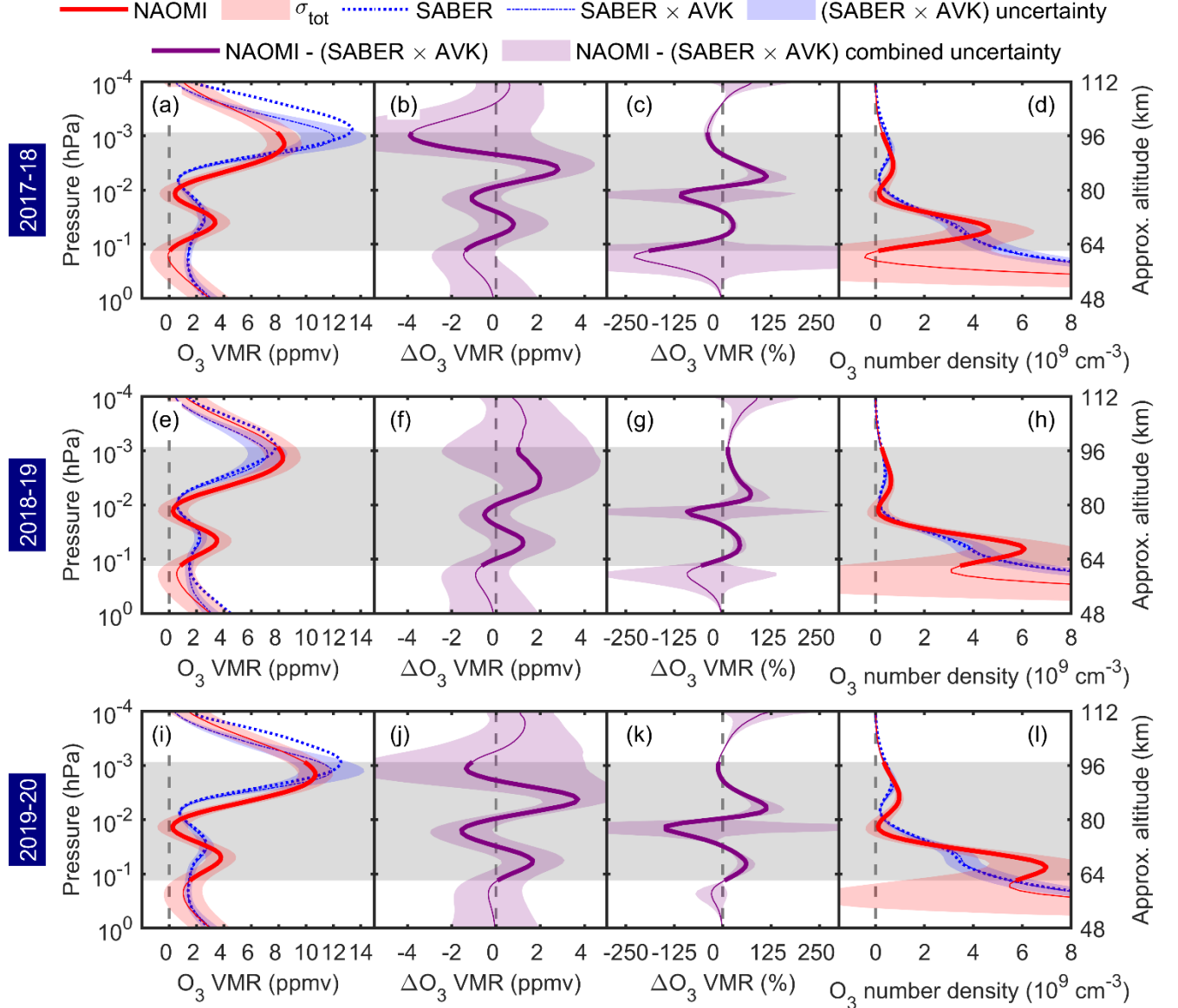
Figure 6: Mean ozone vertical profiles from NAOMI and SABER 9.6 \mu\text{m} observations during winter night-time (within 15 December–15 March, \text{SZA} at altitude 90 km > 110^\circ ) in 2017–18 (a–d), 2018–19 (e–h), and 2019–20 (i–l). The second and third columns give the absolute and relative (%) differences (NAOMI minus SABER 9.6 \mu\text{m} ). The red, blue, and purple shading are the estimated uncertainties of
