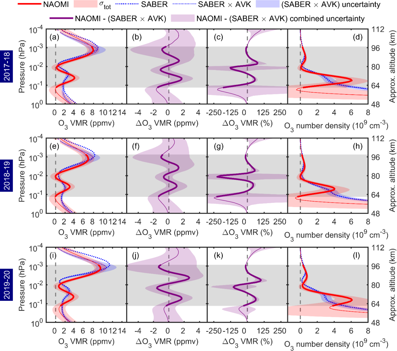
330 Figure 7: Mean ozone vertical profiles from NAOMI and SABER 9.6 \mu\text{m} observations during winter twilight (within 15 December–15 March, 75^\circ \leq \text{SZA} at altitude 90 \text{ km} \leq 110^\circ ) in 2017–18 (a–d), 2018–19 (e–h), and 2019–20 (i–l). The second and third columns give the absolute and relative (%) differences (NAOMI minus SABER 9.6 \mu\text{m} ). The red, blue, and purple shading are the estimated uncertainties of the plotted parameters. The grey shaded regions and thicker sections of the plotted curves indicate the pressure and altitude ranges where MR \geq 0.8 .
