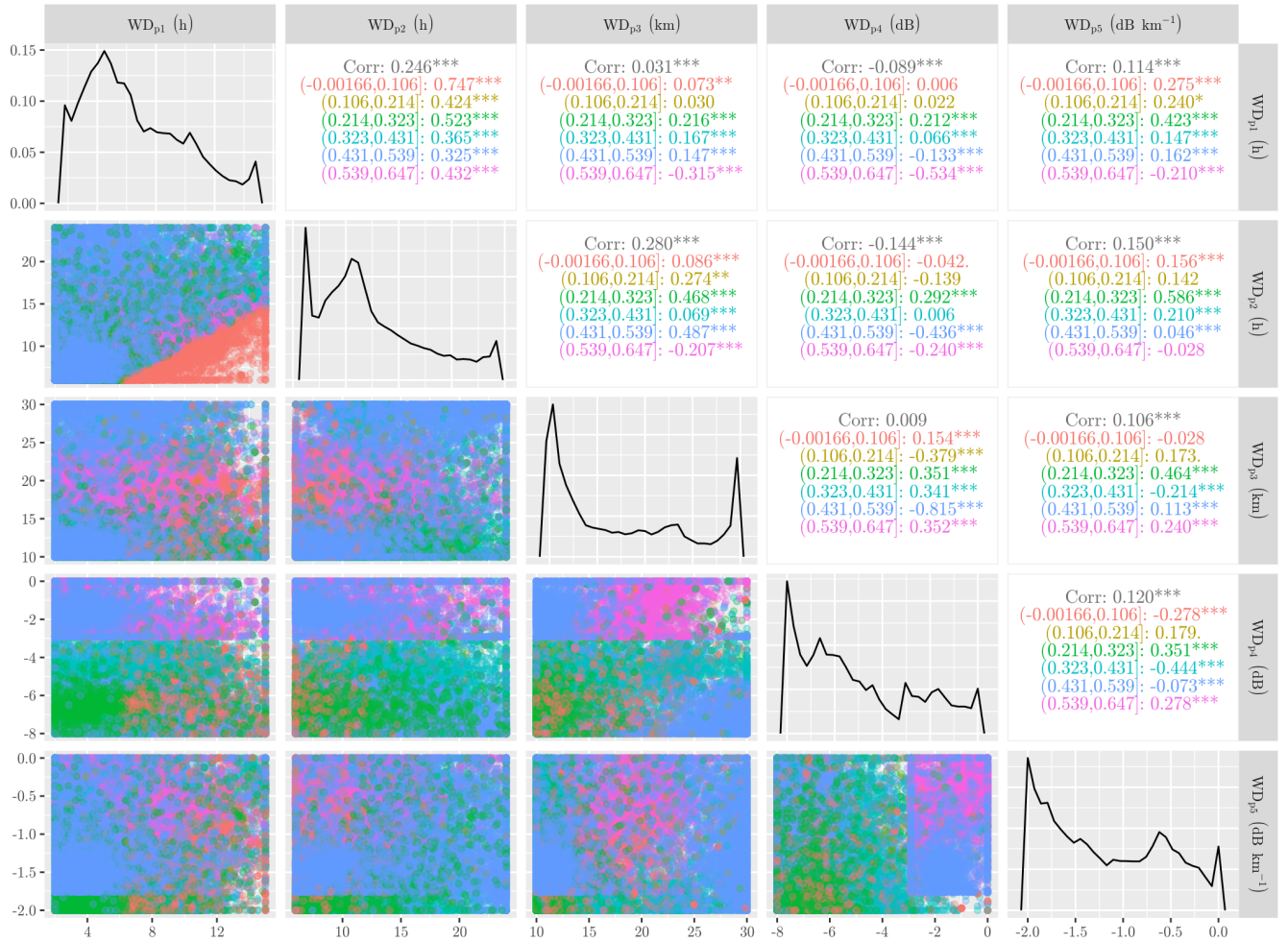
Figure 2. Calibration of the wet-dry classification parameters: (a) dotted plot panel showing the interaction between calibration parameters at different Matthews correlation coefficient (MCC) values; (b) histograms of the parameters.
