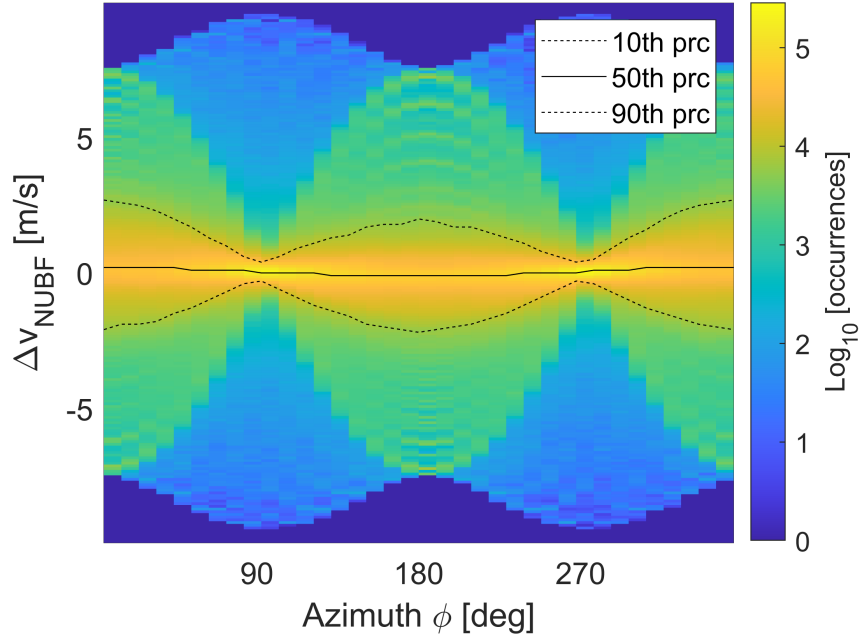
Figure 18. NUBF-induced error as a function of the azimuthal scanning angle. The color modulates indicates the \log_{10} of the number of occurrences. The statistics is computed for 20 orbits over the scene depicted in Figs. 12-15. The dotted lines represent the 10th and 90th percentile (typically with absolute value lower than 2.0 m/s) whereas the continuous line corresponds to the median value (always very close to zero because many NUBF errors are equal and opposite so will tend to cancel out).
