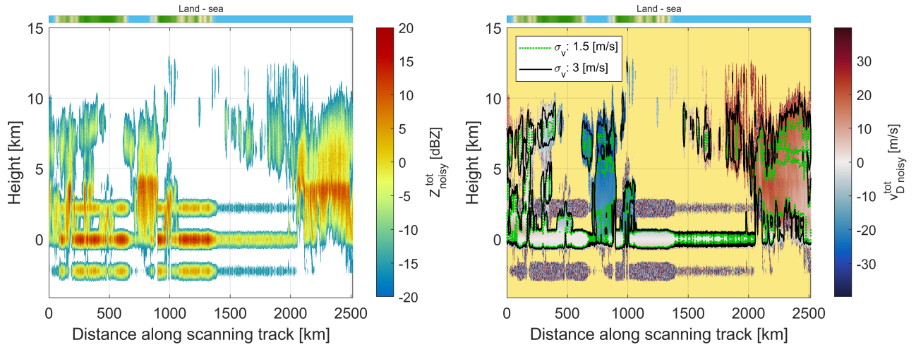
Figure 15. Reflectivities and Doppler results corresponding to a full revolution of the WIVERN antenna as shown in Fig. 13 for an integration length of 1.0 km ( M=8 ). Left panel: simulations of the WIVERN reflectivities (signal+noise) with ghost echoes at 2.3 km above and below the ground due to the depolarisation depolarization by the surface leading to ghost echoes where there is no real cloud. Right panel: WIVERN retrieved line-of-sight Doppler velocities after performing the polarization diversity pulse pair processing. continuous Continuous (dashed) black contour lines correspond to Doppler velocity precision of 3 (1.5) m/s according to Eq. (16)). Note that the ghost ghost -echoes contaminated by ghosts have lower precision.
