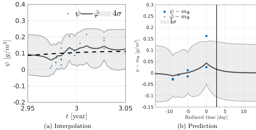
Figure 13. (a) Kriging based interpolation over a period of 36 days centered at the beginning of 3-rd in the dataset. The mean is represented in as a dashed black line ( -- ). (b) Kriging based prediction over a period of \sim 36 days centered at the beginning of 3-rd in the dataset. The vertical black line ( | ) represents the correlation time l_t after the last observation. In (a) and (b), the training set observations are represented as ( \bullet ), the kriging estimate as black line ( - ), and the variance of the estimation error in shaded gray.
