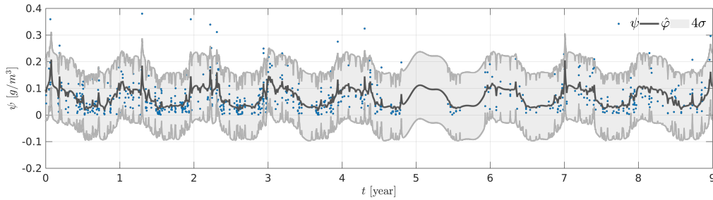
Figure 12. Kriging based interpolation over a 9 year period. The training set observations are represented as ( \bullet ), the kriging estimate as ( - ), and variance of the estimation error (shaded gray).
