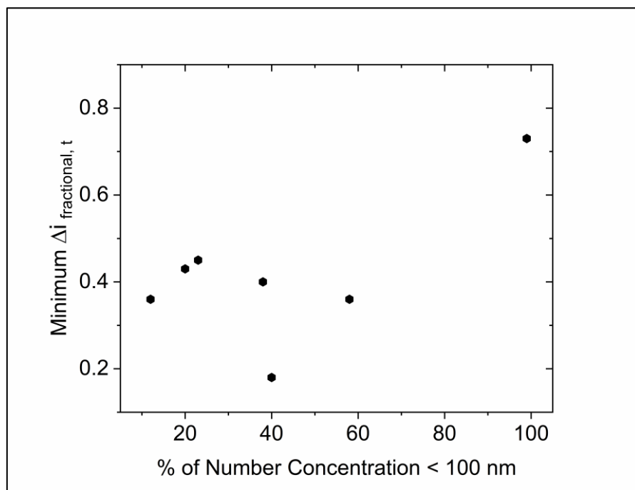
325 Figure 9. Minimum \Delta i_{\text{fractional}, t} as a function of percentage of number concentration of particles (within a distribution) below 100 nm in aerodynamic diameter.
