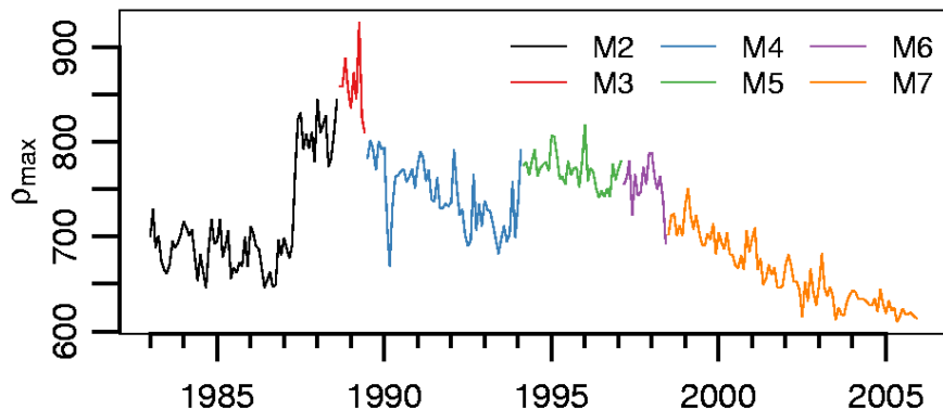
Figure 4. Temporal evolution of the 95th percentile ( \rho_{max} ) of the observed reflections for MVIRI, covering 1983 to 2005. The different MVIRI instruments (M 2-7) are coloured for a better distinction. Image from Posselt et al. 2011
