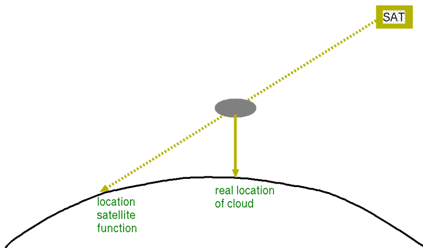
Figure 5. Illustration of the parallax effect.
