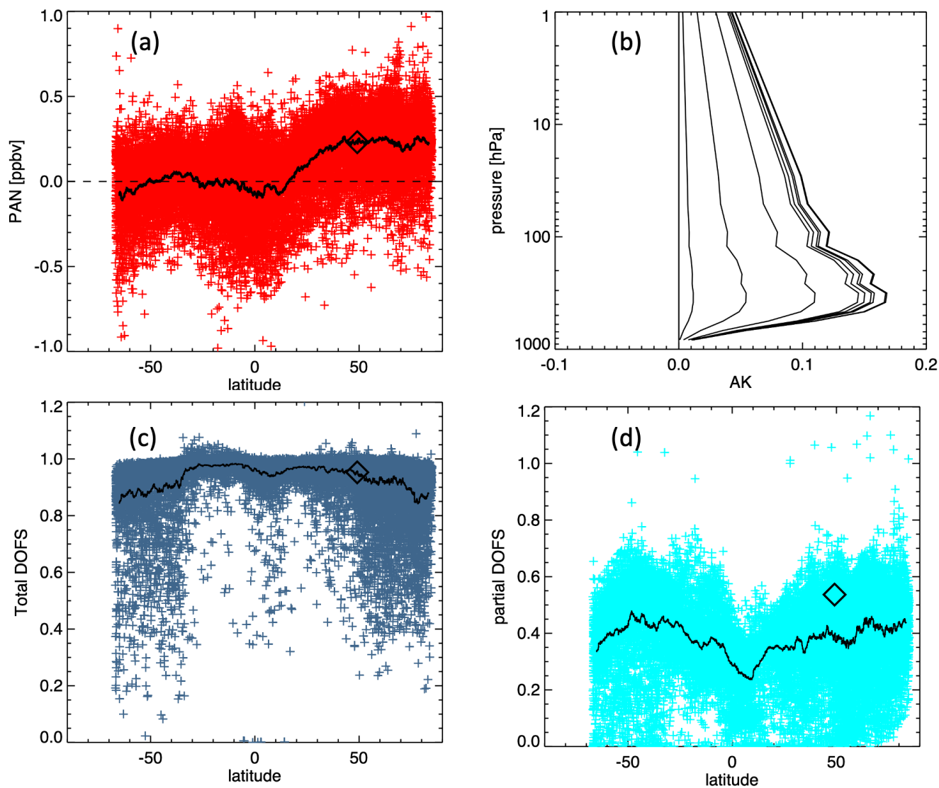
590 Figure 6. (a) CrIS PAN retrievals for sub-sampled measurements for 1st August 2020, plotted by latitude. Black solid line shows a 595 running mean over a 200 point window. (b) Averaging kernel for an example mid-latitude case (from a point at the center of the black diamond shown in (a), (c) and (d). Panels (c) and (d) show total and partial (825-316 hPa) DOFS for retrievals from this day.
