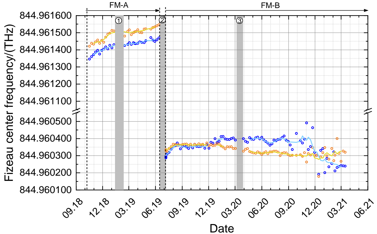
Figure 10. Fizeau center frequency derived from the direct channel (blue circles) and the reflected channel (orange circles) by fitting Eq. (9) and Eq. (11) to the ISR data sets obtained from October 2018 to March 2021 (see also table 2). The corresponding moving average of five successive data points is indicated by the light blue line and yellow line, respectively. Special time periods are indicated by gray bars (1 = Instrument shut-off due to a GPS reboot anomaly, 2 = switch from FM-A to FM-B, 3 = Laser CPT optimization).
