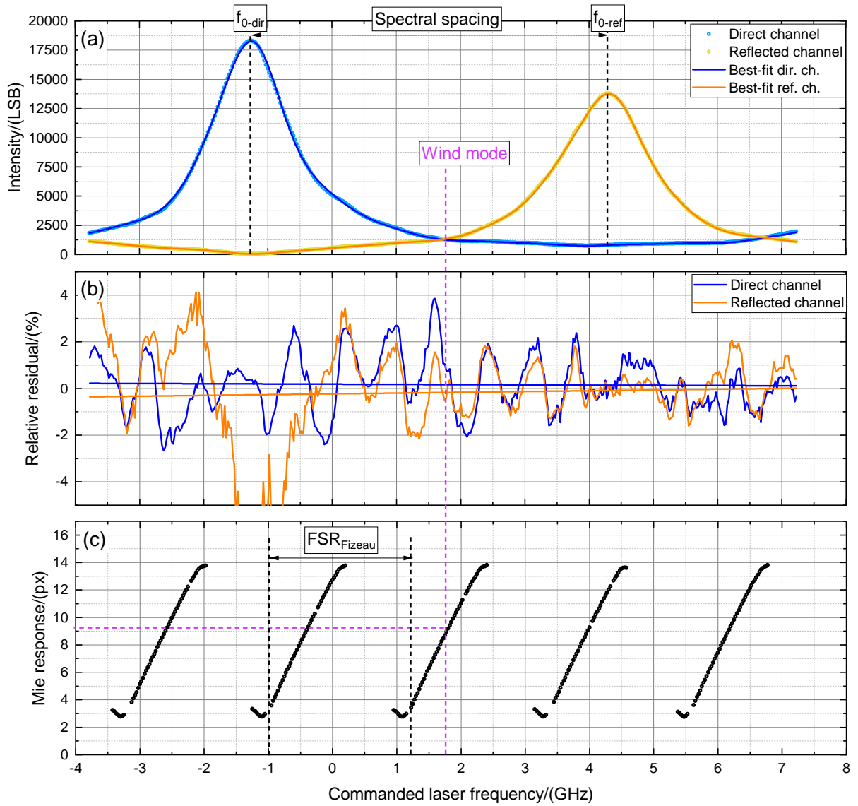
Figure 5. (a): FPI transmission curves of the direct channel (light blue dots) and the reflected channel (yellow dots) measured on 10 October 2018 being laser energy corrected by means of E_{\text{norm}_{\text{new}}}(f) (see also Eq. (2)), and the corresponding best-fits according to Eq. (9) and Eq. (11) in blue (direct channel) and orange (reflected channel), respectively. (b): Related relative residuals of the direct channel (blue) and reflected channel (orange). (c): Corresponding Mie response, i.e. the fringe center position on the ACCD pixel.
