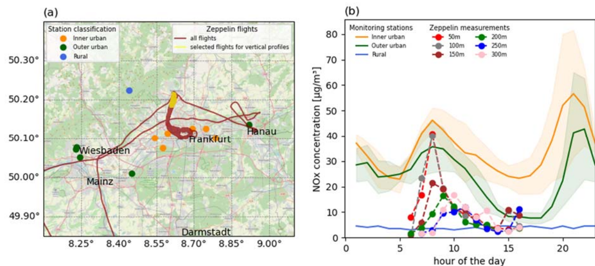
Figure 4: a. The map of Frankfurt overlaid with the Zeppelin flight tracks in red and yellow that are used to generate the vertical profiles shown on the right. Multiple flight paths to the city center of Frankfurt are overlaid and appear as a thick red
